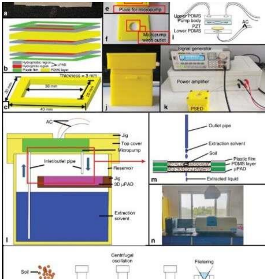
Picture of an integrated soil–liquid extraction device. (a) Physical picture of the 3D \mu PAD. (b) Structural picture of the 3D \mu PAD. (c) Size of the PDMS layer. (d) Jig of the \mu PAD. (e) Top cover. (f) Jig of the micropump. (g) Reservoir. (h) Physical picture of the micropump. (i) Composition of the micropump. (j) Assembled PSED. (k) Experimental platform of the PSED. (l) The inner structure of the PSED. (m) Experimental principle of the PSED. (n) Fire atomic absorption spectrometer (FASS). (o) Experimental principle of traditional soil–liquid extraction.
