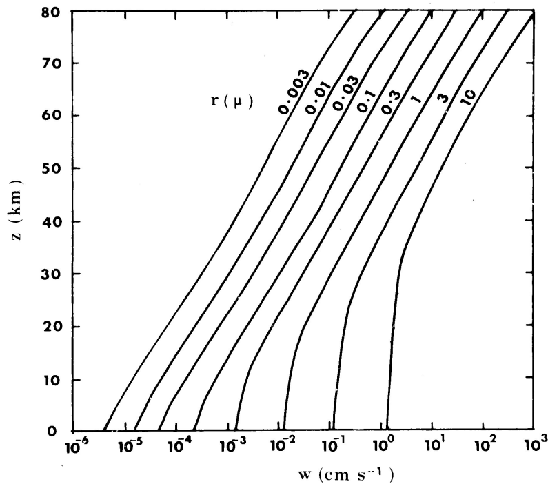
Figure. 5 . Falling speed of spherical dust particles as a function of height in the atmosphere (reproduced from Hoyle & Wickramasinghe (10), Proofs that Life is Cosmic , Mem. Inst.Fund.Studies, Sri Lanka, 1982) (copyright Chandra Wickramasinghe)
