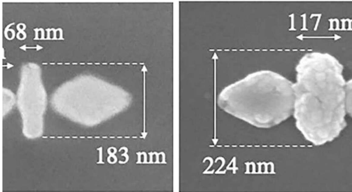
Scanning electron microscope images of the nano-butterfly structure before (left) and after (right) laser irradiation. Semiconductor zinc oxide has crystallized on the surface of the gold nanorod. Credit: Fujiwara H., et al, Nano Letters. December 23, 2019
