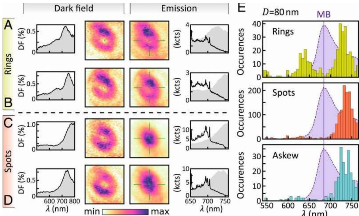
Comparison of ring and spot emission from 80-nm NPoMs. (A–D) From left to right: Dark-field spectra, dark-field image, emission image, and emission spectra for NPoMs exhibiting rings (A and B) and spots (C and D). (E) Analysis of scattering spectra peak central wavelengths classed by shape, for 1,602 NPoMs. Shaded gray curves in emission spectra (A–D) are same dark-field (DF) spectra. Purple shaded curves in E show the MB dye emission in solution. Credit: PNAS, doi: https://doi.org/10.1073/pnas.1914713117
