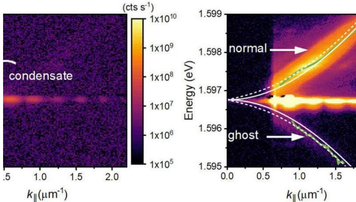
Left: momentum-space luminescence of the strong signal from the high-density condensate. Right: same data taken with a razor-edge filter covering the signal from the condensate, revealing the normal and ghost excitations of the condensate. Credit: FLEET
