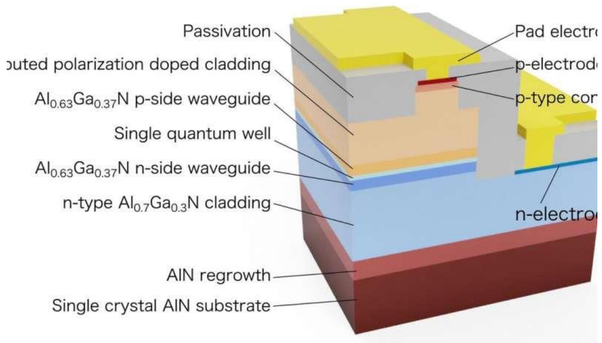
Cross-sectional structure of the UV-C semiconductor laser diode. Credit: 2019 Asahi Kasei Corp. and Nagoya University
