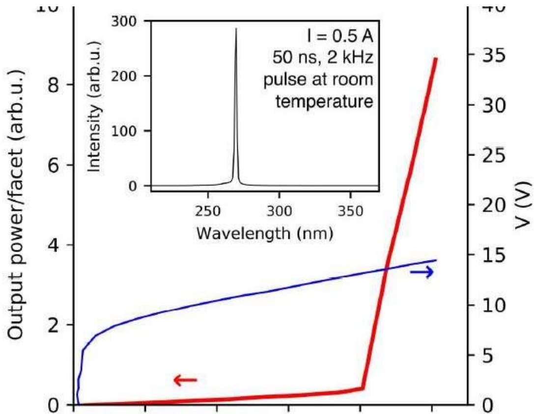
Emission characteristics under pulsed operation. Credit: 2019 Asahi Kasei Corp. and Nagoya University
