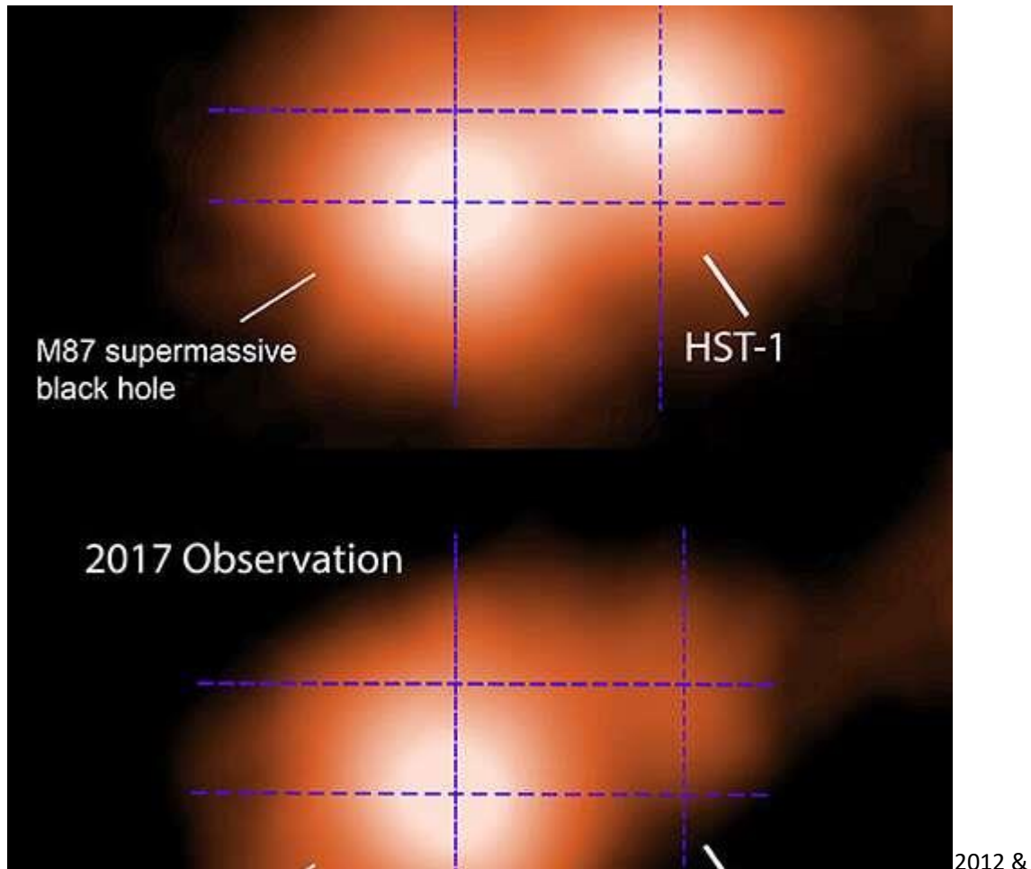
2012 & 2017 Labeled Insets. Credit: NASA/CXC/SAO/B. Snios et al.
