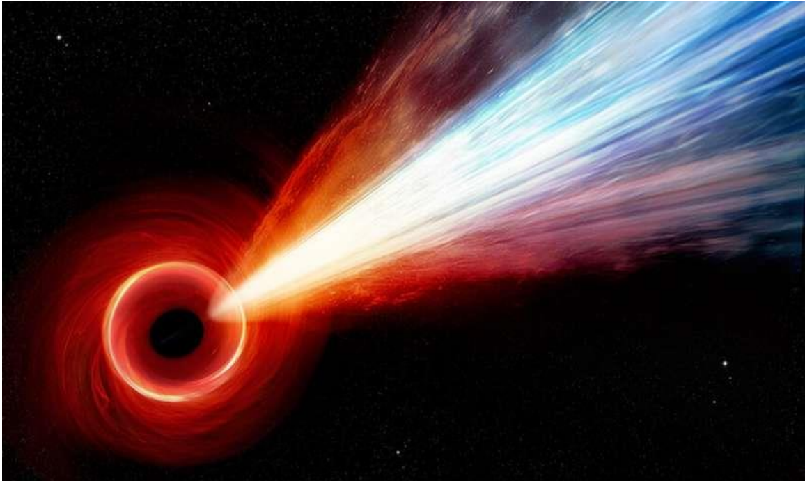
Illustration of the Supermassive Black Hole at the Center of M87. Credit: NASA/CXC/M.Weiss
