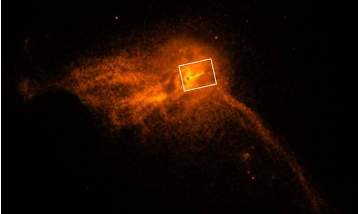
Chandra Wide-field View of M87; box shows the approximate location of the wide-field jet image above. Credit: NASA/CXC
