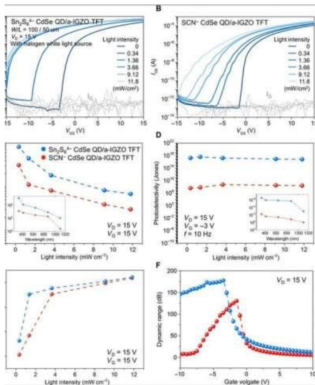
LEFT: Optoelectronic performance of the QD/AOS hybrid phototransistor. Photoresponse characteristics of the QD/a-IGZO phototransistor with (A) \text{Sn}_2\text{S}_6^{4-} and (B) \text{SCN}^- ligands. (C) Photosensitivity ( R ) and (D) photodetectivity ( D^* ) under white light ( 1.36 \text{ mW cm}^{-2} ) and broadband illumination (inset). Light intensities of UV, blue, green, and red are 1 \text{ mW cm}^{-2} , while that for IR is 13.6 \text{ mW cm}^{-2} and that for white light is 1.36 \text{ mW cm}^{-2} . (E) EQE and (F) dynamic range of 7-nm CdSe QD/a-IGZO with the \text{Sn}_2\text{S}_6^{4-} ligand (blue line) and the \text{SCN}^- ligand (red line) phototransistor. Photo credit: Jaehyun Kim, Displays and Devices Research Lab. School of Electrical and Electronics Engineering, Chung-Ang University, Seoul 06974, Korea. RIGHT: Fine-patterned QDs characteristics. (A) Schematic representation of QDs to design photosensitive inorganic ligands. (B) Optical and (C) field-enhanced scanning electron microscopy (FESEM) images of patterned CdSe QDs capped with \text{Sn}_2\text{S}_6^{4-} ligands. (D) CdS QDs, (E) PbS QDs. Scale bars, 100 \mu\text{m} (B), 5 \mu\text{m} (C), 20 \mu\text{m} (D), and 10 \mu\text{m} (E). (F and G) Atomic force microscopy (AFM) scan image and height profile of CdSe QDs from along the blue dashed line. Scale bar, 5 \mu\text{m} . Photo credit: Jaehyun Kim, Displays and Devices
