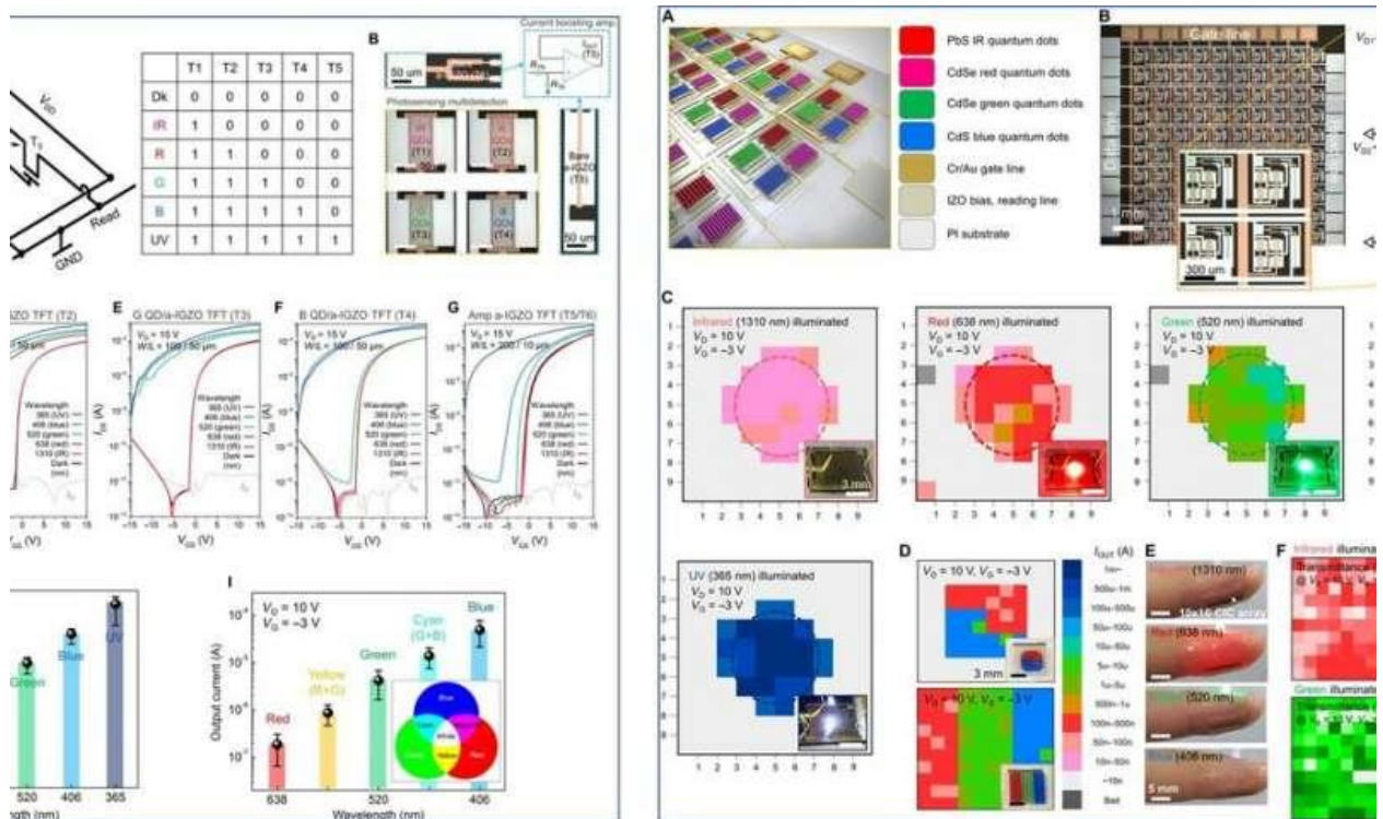
LEFT: CIC array characteristics for full-color discrimination. (A) Schematic diagram of CIC and logic table of full-color signal detection in one pixel. (B) Optical micrograph of the partially patterned QDs including IR PbS (T1, 10 nm), red CdSe (T2, 7 nm), green CdSe (T3, 5 nm), and blue CdS (T4, 3 nm) and bare a-IGZO phototransistors and the schematic of amplification circuit. RTN is the channel resistance of load TFTs (T1 to T4), and RT6 is the channel resistance of driver TFT (T5). Here, channel width/length are 100/50 \mu\text{m} (load TFTs), 200/10 \mu\text{m} (T5), and 5/200 \mu\text{m} (T6). Scale bar, 50 \mu\text{m} . (C to G) Photoresponse characteristics of T1, T2, T3, T4, and T5/T6 with respect to wavelength of light. (H) Output current of the five-channel full-color
