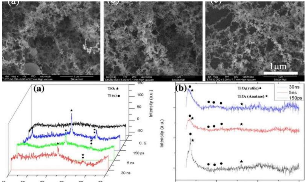
TOP: SEM images of NFTi layer (Nanofibrous Titania) with power = 10 W, frequency = 600 KHz (a) pulse duration = 150 ps, (b) pulse duration = 5 ns, (c) pulse duration = 30 ns with 50000X magnification. BOTTOM: (a) XRD pattern, (b) Raman spectrum of bare glass and samples coated by titania with different pulse durations (created by Origin Pro 2019B (GF3S4-3089-7907079) https://www.originlab.com/ ). Credit: Scientific Reports, doi: 10.1038/s41598-019-54533-z.
