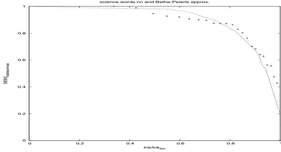
FIG. 49. Vertical axis is \frac{\ln f}{\ln f_{\text{nextnext-max}}} and horizontal axis is \frac{\ln k}{\ln k_{\text{lim}}} . The + points represent the words of the dictionary of science with fit curve being Bethe-Peierls curve in presence of four nearest neighbours.
