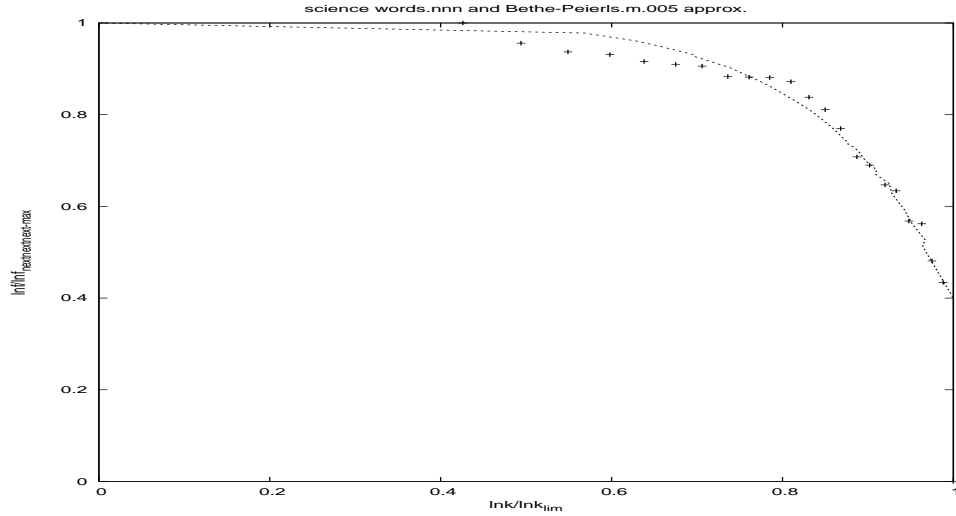
FIG. 50. Vertical axis is \frac{\ln f}{\ln f_{\text{nextnext-max}}} and horizontal axis is \frac{\ln k}{\ln k_{\text{lim}}} . The + points represent the words of the dictionary of science with fit curve being Bethe-Peierls curve in presence of four nearest neighbours in presence of magnetic field m = 0.005 or, \beta H = 0.01 .
