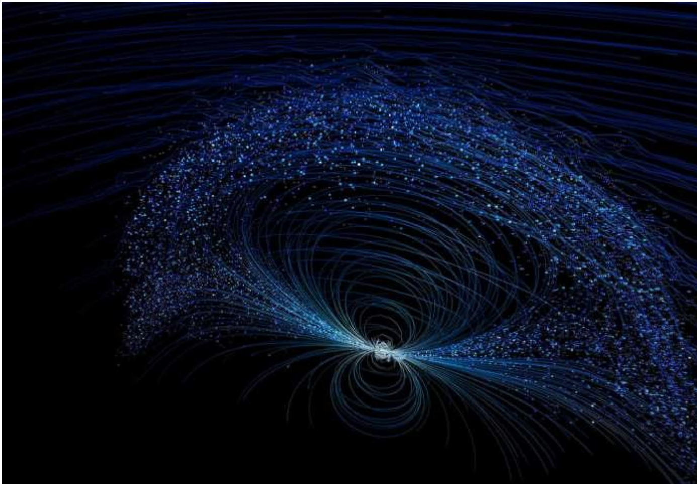
The OSIRIS computer model predicts how powerful magnetic fields around pulsars evolve, helping scientists understand where matter and antimatter can be created out of the vacuum of space. Credit: Fabio Cruz
