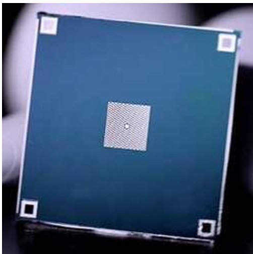
A thin silicon nitride membrane (white) is stretched tight across a silicon frame (blue). The membrane contains a pattern of holes, with one small island in the center, whose vibrations are measured in the experiment. Credit: Niels Bohr Institute
