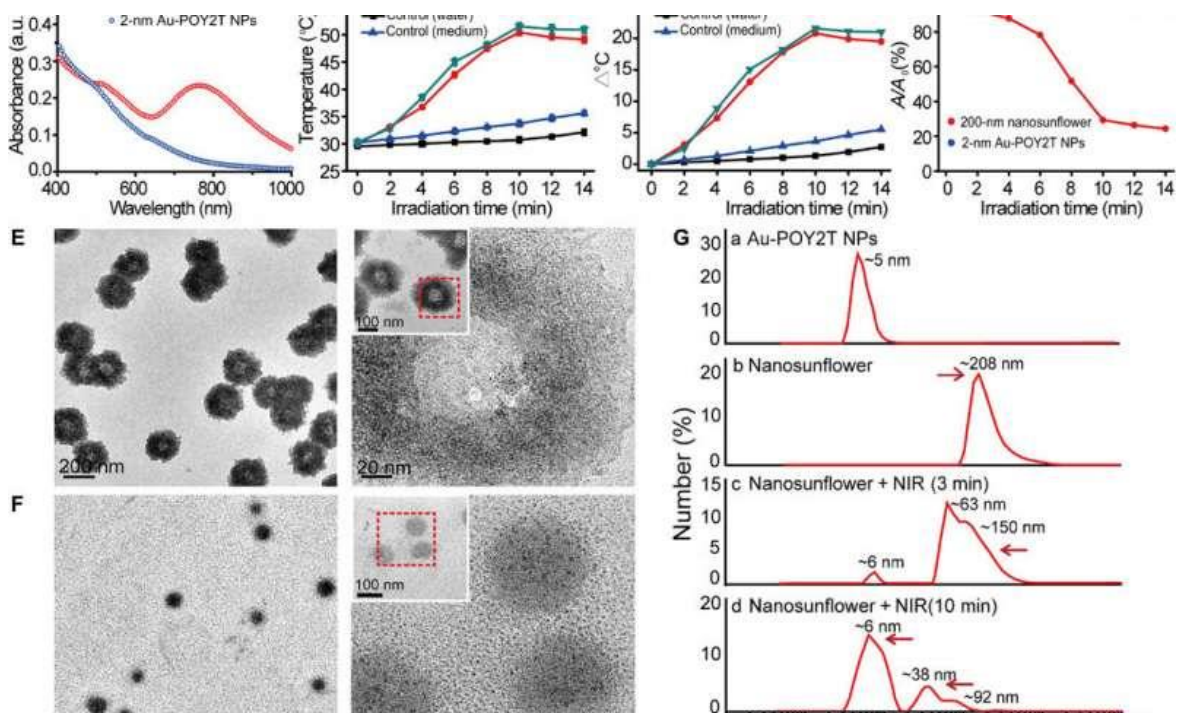
Photothermal property and disassembly behavior study of the self-assembled nanostructures. (A) Visible absorption spectra of 2-nm core-sized NPs and 200-nm self-assembled nanostructures. a.u., absorbance unit. (B) Temperature response of self-assembled nanostructures, upon NIR irradiation, dispersed in water and cell culture medium. Mean values \pm SD, n = 3 . (C) Temperature rise of self-assembled nanostructures, upon NIR irradiation, dispersed in water and cell culture medium. (D) Change of maximum absorbance (767 nm) of 2-nm core-sized NPs and 200-nm self-assembled
