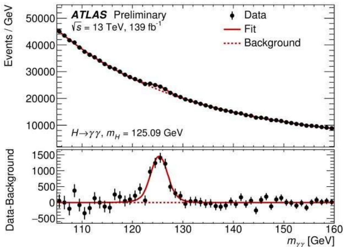
Figure 3: Distribution of the invariant mass of the two photons elected in the ATLAS measurement of H \rightarrow \gamma\gamma using the full Run 2 dataset. The Higgs boson corresponds to the excess of events observed at 125 GeV with respect to the non-resonant background (dashed line). Credit: ATLAS Collaboration/CERN
