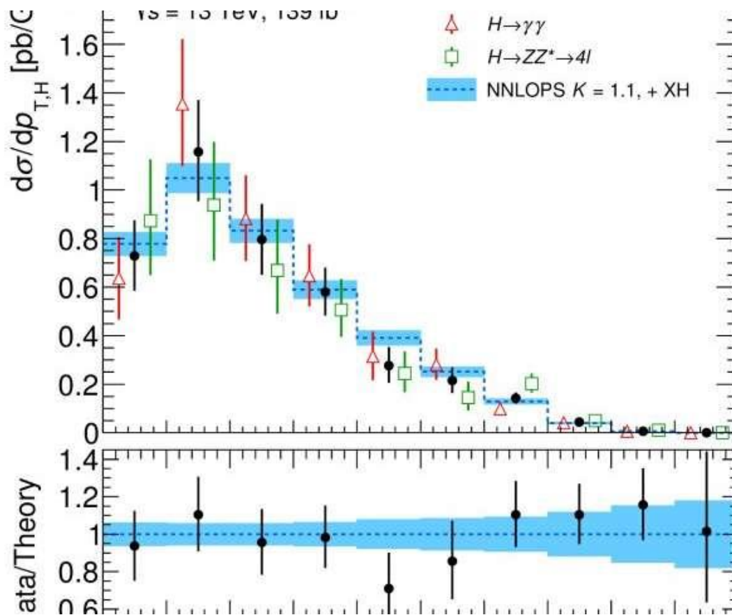
Figure 4: Differential cross section for the transverse momentum ( p_{T,H} ) of the Higgs boson from the two individual channels ( H \rightarrow ZZ^* \rightarrow 4\ell , H \rightarrow \gamma\gamma ) and their combination. Credit: ATLAS Collaboration/CERN
