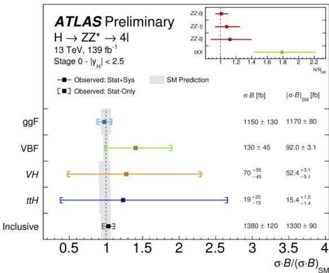
Figure 2: The Higgs production cross sections times the Higgs branching fraction into a pair of Z bosons, \sigma \cdot B , as measured in the four-lepton decay channel. These are normalised by the Standard Model expected values. The vertical line at one is the Standard Model expectation with the grey band corresponding to the theory uncertainties on this expectation. The measured data points agree well within their uncertainties with the Standard Model. Credit: ATLAS Collaboration/CERN
