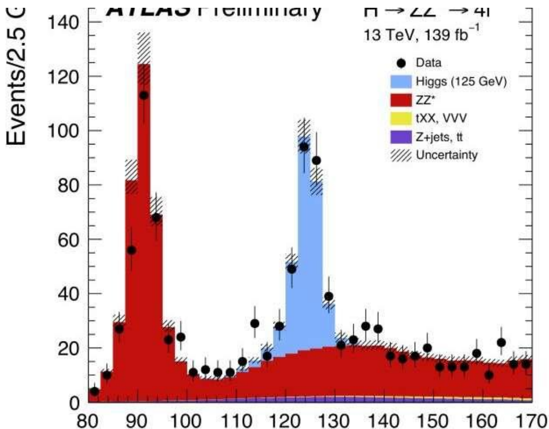
Figure 1: Distribution of the invariant mass of the four leptons selected in the ATLAS measurement of H \rightarrow ZZ^* \rightarrow 4\ell using the full Run 2 dataset. The Higgs boson corresponds to the excess of events (blue) over the non-resonant ZZ^* background (red) at 125 GeV. A rare Z boson decay into four leptons can also be observed at about 91 GeV. Credit: ATLAS Collaboration/CERN
