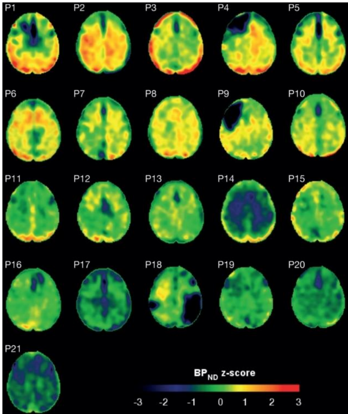
Brain scans showing the amount of tau protein in the brains of patients who have suffered a traumatic brain injury compared voxel-wise to healthy controls. Red represents increased tau accumulation. (Courtesy: Gorgoraptis et al/Science Transitional Medicine)
