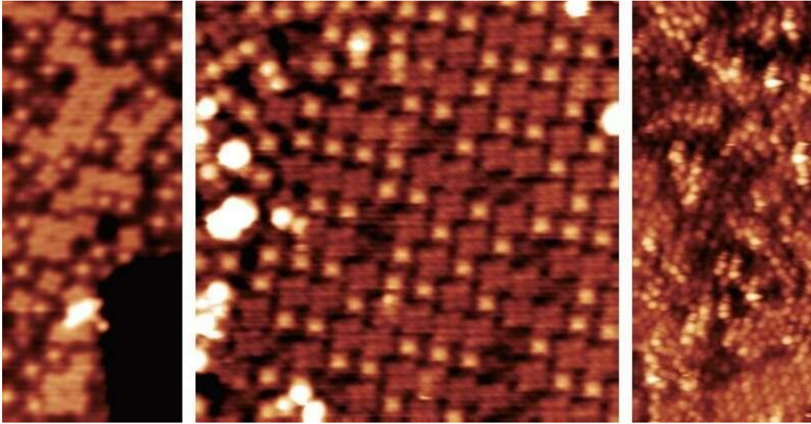
Scanning tunneling microscopy images of the organic layer at 0.6 molecule thick (left), 1.0 molecule thick (center) and 1.9 molecules thick (right). Credit: © 2019 Isshiki et al.
