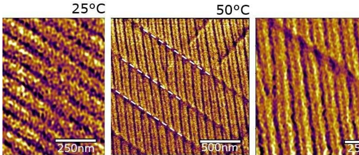
Domain walls in barium titanate at increasing temperature (please note different scales). Credit: Noheda lab
