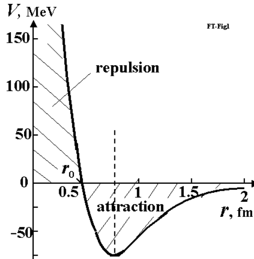
Fig.8. Typical nuclear force of nucleus. When nucleon is at distance of less than 1.8 fm, it is attracted to nucleus. When nucleon is very close, it is repulsed from nucleus.
