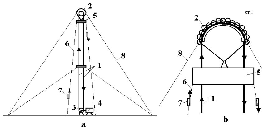
Fig.5. a. Offered kinetic tower: 1 – mobile closed loop cable, 2 – top roller of the tower, 3 – bottom roller of the tower, 4 – engine, 5 – space station, 6 – elevator, 7 – load cabin, 8 – tensile element (stabilizing rope). b. Design of top roller.
