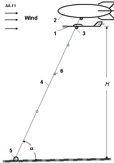
Fig.2. High altitude aerial antenna. Notations: 1 – special high lift air apparatus; 2 – small dirigible (air balloon) for supporting the aerial antenna at high altitude; 3 – high altitude antenna; 4 – cable; 5 – winch; 6 – illuminations and sensor of wind intensity.
