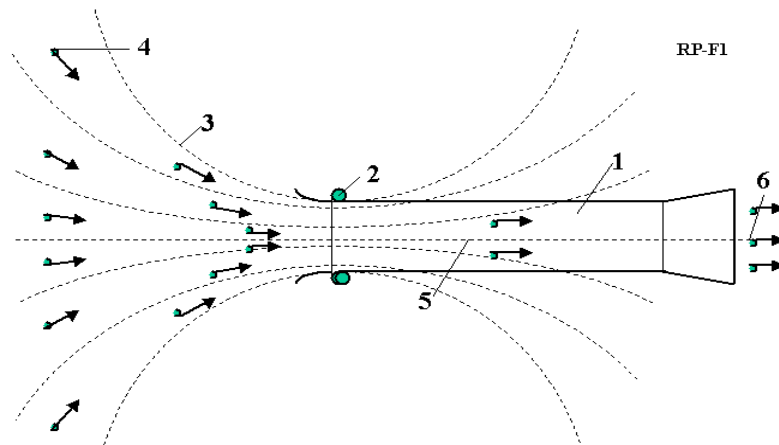
Fig. 16.1. Recombination space jet propulsion engine (actuator of magnetic field). Notations are: 1 – engine, 2 – solenoid, 3 – magnetic lines, 4 – charged particles, 5 – recombination zone, 6 – exit.
