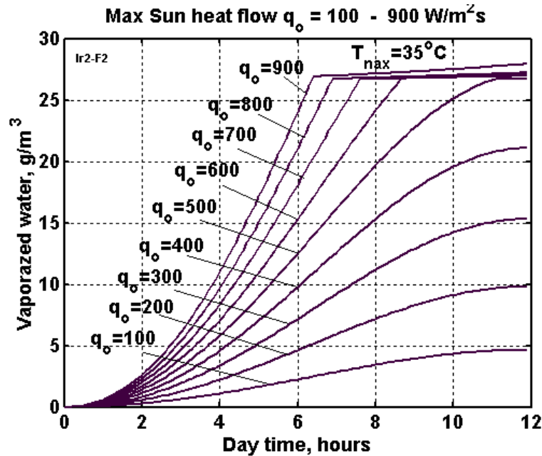
Fig.11. Water vaporization for 100% humidity of the air for different maximal solar radiation ( W/m^2 ) levels delivered over varying daily time. Height of dome film cover equals H = 135 m. The temperature control system limits the maximum internal dome temperature to 35 C.
