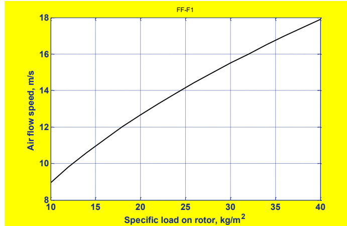
Fig.9. Air speed of a helicopter jet under the helicopter rotor (propeller) via specific load on helicopter rotor.
