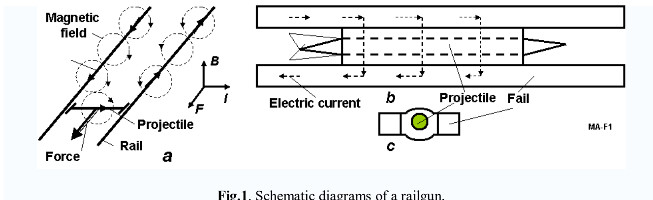
Fig.1. Schematic diagrams of a railgun.
