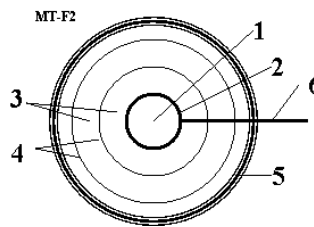
Fig.3. Cross-section of superconductive tube. Notations: 1 - strong tube (internal part used for cooling of ring, external part is used for superconductive layer; 2 - superconductive layer protected the insulator and heat protection; 3 - vacuum; 4 – heat impact reduction high-reflectivity screens (roll of thin bright aluminum foil); 5 - protection and heat insulation and high reflective layer, 6 – outer electric contact for control system and climber.
