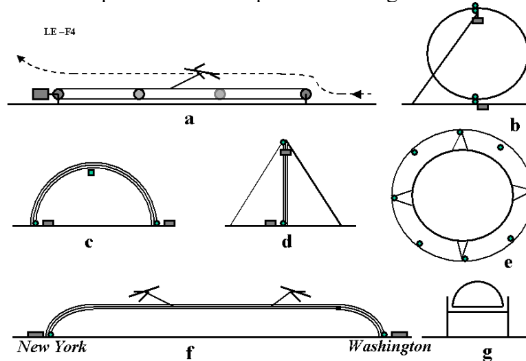
Figure 7-1. Installations needing the linear electrostatic engine. (a) Space cable launcher [2]; (b) Circle launcher; (c) Space keeper [1]; (d) Kinetic space tower[1]; (e) Earth round cable space keeper [1]; (f) Cable aviation [1]; (g) Levitation train [1].
