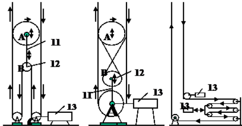
Fig. 1-2. Two mechanisms for changing the rope length in the Transport System (They are same for the space station). Notations: 11 - the rope which is connected axis A,B . This rope can change its length (the distance AB ); 12 - additional rollers.
