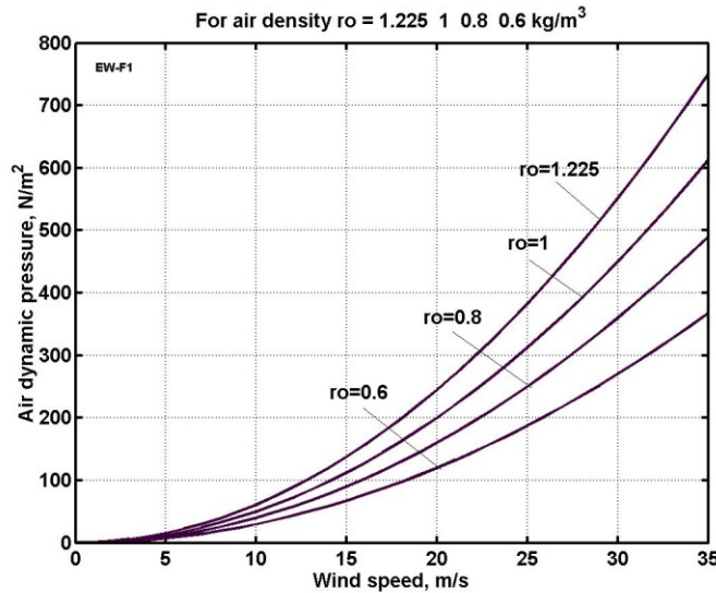
Fig. 18. Wind dynamic pressure versus wind speed and air density \rho . The \rho = 0.6 is for H \approx 6 km.
