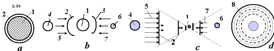
Fig.3. Cross-section of superconductive tube. Notations: 1 - strong tube (internal part used for cooling of ring, external part is used for superconductive layer; 2 - superconductive layer protected the insulator and heat protection; 3 - vacuum; 4 – heat impact reduction high-reflectivity screens (roll of thin bright aluminum foil); 5 - protection and heat insulation and high reflective layer, 6 – outer electric contact for control system and climber.
