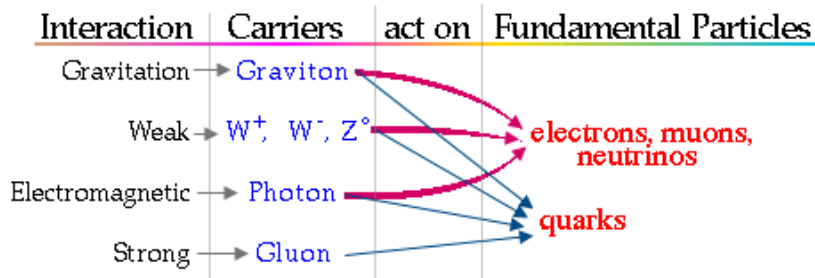
Fig.5. Interaction between fundamental particles.
