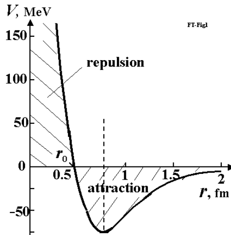
Fig. 16-1. Typical nuclear force of nucleus. When nucleon is at distance of less than 1.8 fm, it is attracted to nucleus. When nucleon is very close, it is repulsed from nucleus.
