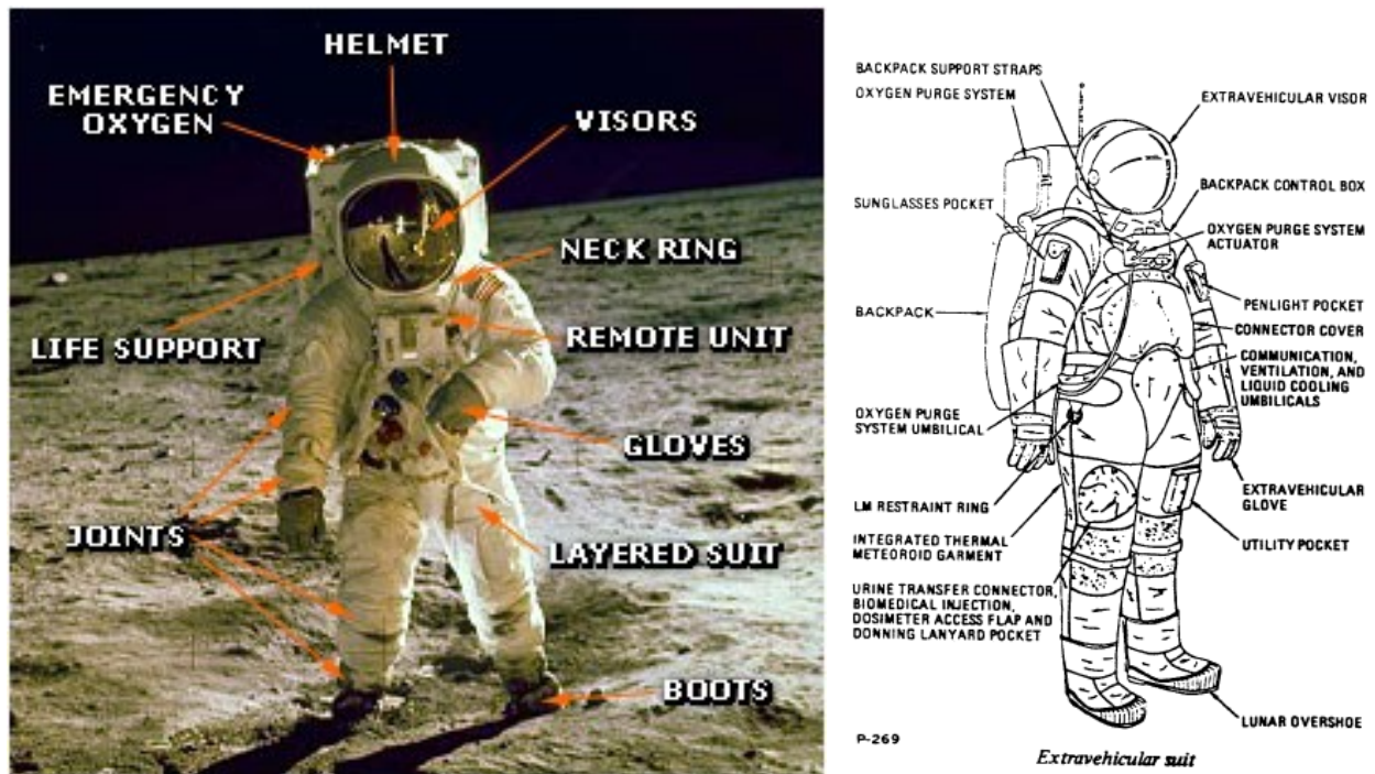
Fig. 1. a. Apollo 11 A7L space suit. b. Diagram showing component parts of A7L space suit.
