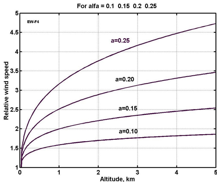
Fig. 12. Relative wind speed versus altitude for V_o = 6 m/s, H_o = 10 m/s.
