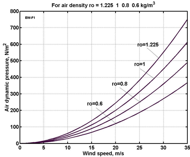
Fig. 4. Wind dynamic pressure versus wind speed and air density \rho . The \rho_0 = 0.6 is for H \approx 6 \text{ km} .
