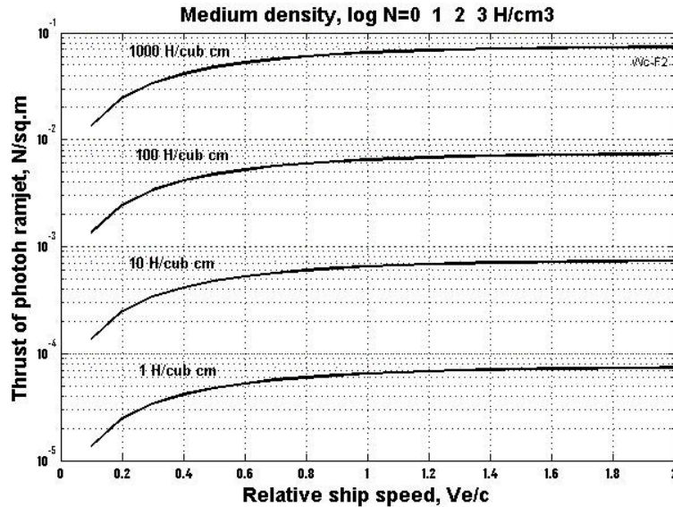
Fig.10. Thrust of photon ramjet engine via relative ship speed v_e/c and number protons (H) in 1\text{cm}^3 .
