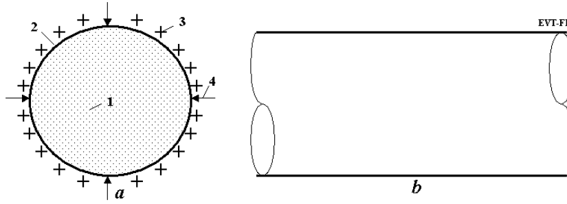
Fig.3. Electronic vacuum AB-Tube. a) Cross-section of tube. b) Side view. Notation: 1 – Internal part of tube filled by free electrons; 2 – insulator envelope of tube; 3 – positive charges on the outer surface of envelope (over this may be an additional film-insulator); 4 – atmospheric pressure.
