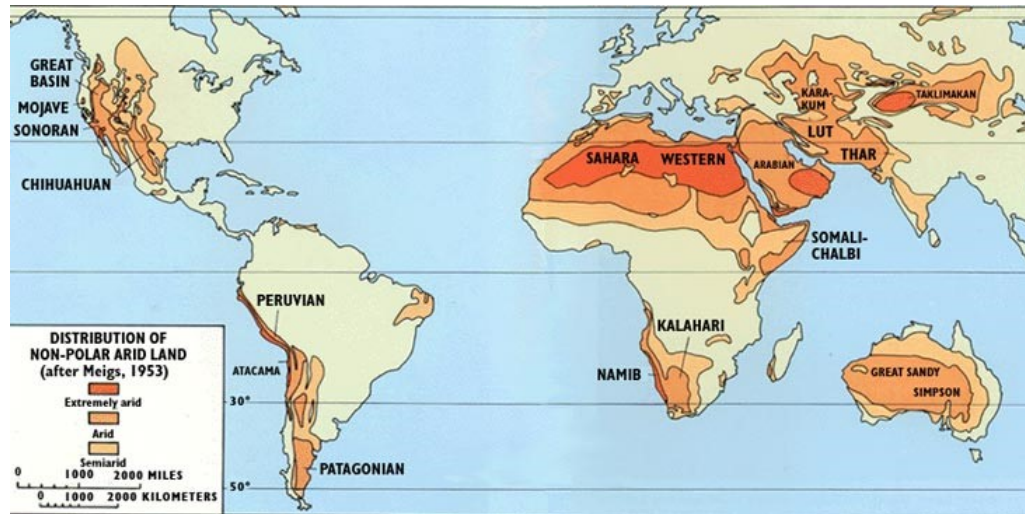
Fig. 1. Distribution non-polar arid land. 78 kb
