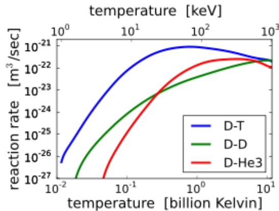
Fig.2. Reaction rate \langle \sigma v \rangle via plasma temperature for D-T (top), D-D (middle) and D- {}^3\text{He} (bottom in left side).
