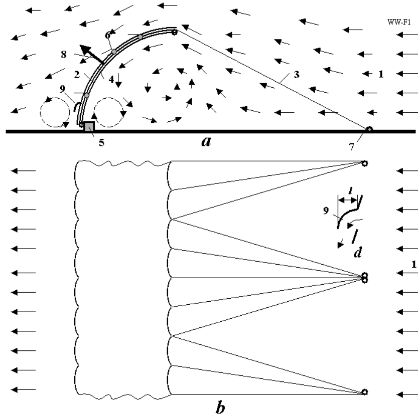
Fig. 4. Fabric AB-Wind Wall of a semi-parachute form. a) Side view, b) Top view, d) Lift hole. Notation: 1 – wind; 2 – fabric wall, 3 – support cable (it may has support wing); 4 – water tube for rain; 5 – water electric station; 7 – control of wall height, 8 - summary drag-lift force of wall; 9 – lift hole. Wall height is about 3 – 5 km.
