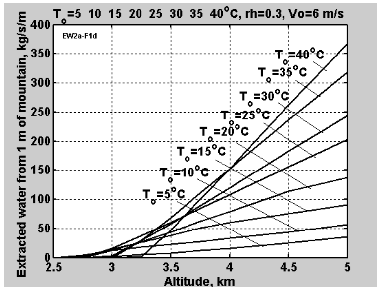
Fig. 13. Amount of water flow may be extracted by 1 m of the AB-Wall (rain and wall) via wall height for different air temperature T_0 at H_0 = 10 m, air speed V_0 = 6 m/s, relative air humidity rh = 0.3 at sea level. Collector efficiency k_c = 1 , coefficient increasing of air speed with altitude \alpha = 0.15 ; H_m = 5 km. The part of this water is realized as rain before Wind Wall and part is precipitations on wall surface ( k_c < 1 ).
