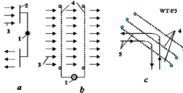
Figure 5-3. Getting the plasma current energy from plasma cable. a - getting by two thin conducting films; b - getting two nets which brake the electric current flux; c - plasma reflector. Notations: 1 - spaceship or space station, 2 - set (films) for collect (emit) the charged particles, 3 - plasma cable, 4 - electrostatic nets.
