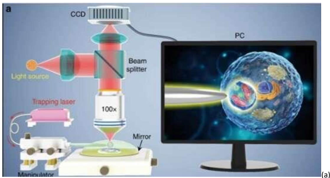
Schematic illustration of the experimental setup. A conventional reflection-mode microscope
