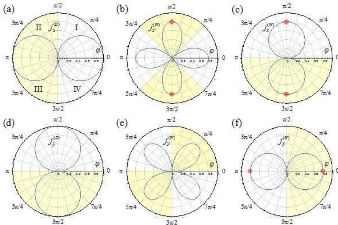
Angular patterns of the x- and y- components of the conventional (a, d), warping (b, e) and Hall (c, f) electric current density. Yellow shading marks the areas of negative current (directed opposite to
