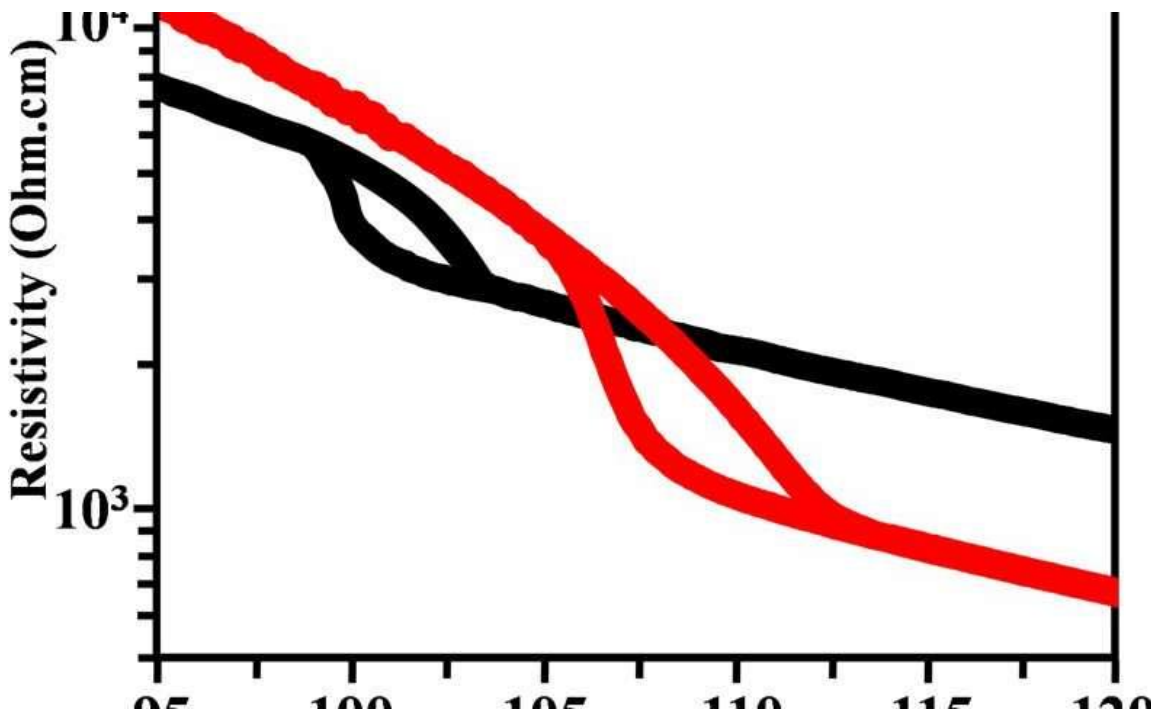
Fig. 3 Transport properties for the nanowire (red) and the film (black) samples. The nanowire showed about six times larger resistance change through Verwey transition. Credit: Osaka University
