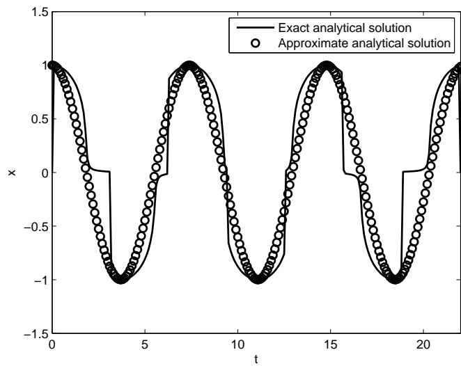
Figure 2: Comparison of the solution (4.11) with (4.12)
