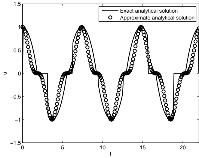
Figure 1: Comparison of the solution (4.2) with (4.7)
