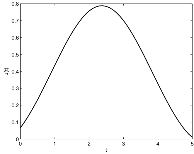
Figure 3: Behavior of the solution (4.43)
