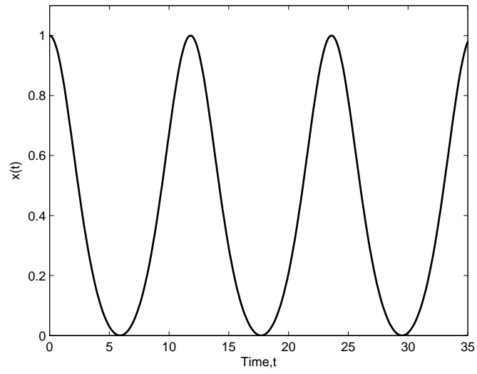
Figure 7: Typical behavior of the solution (4.71)
