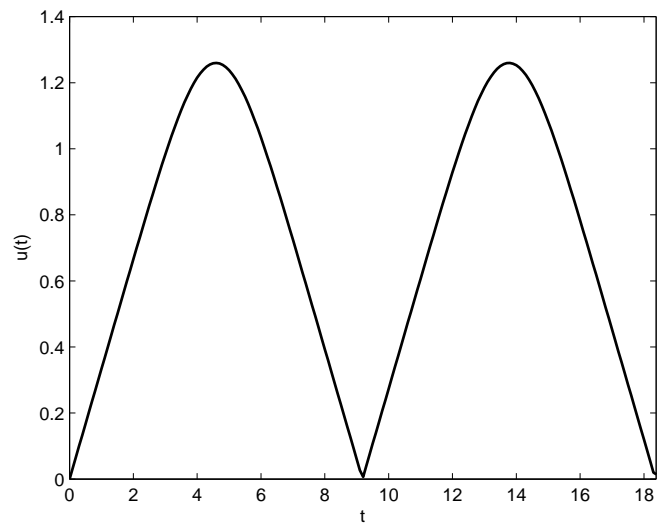
Figure 4: Typical behavior of the solution (4.54)
