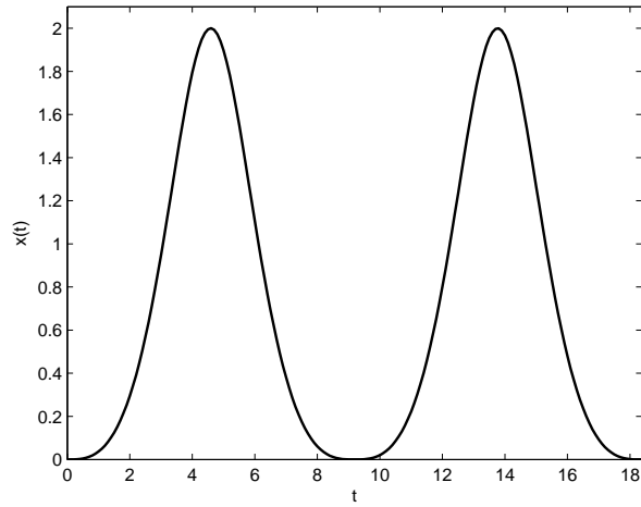
Figure 5: Typical behavior of the solution (4.60)
