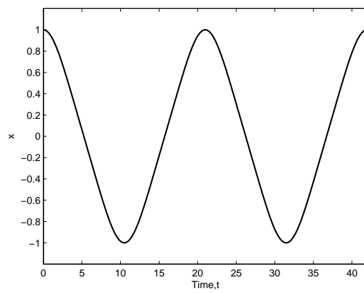
Figure 6: Typical behavior of the solution (4.67)
