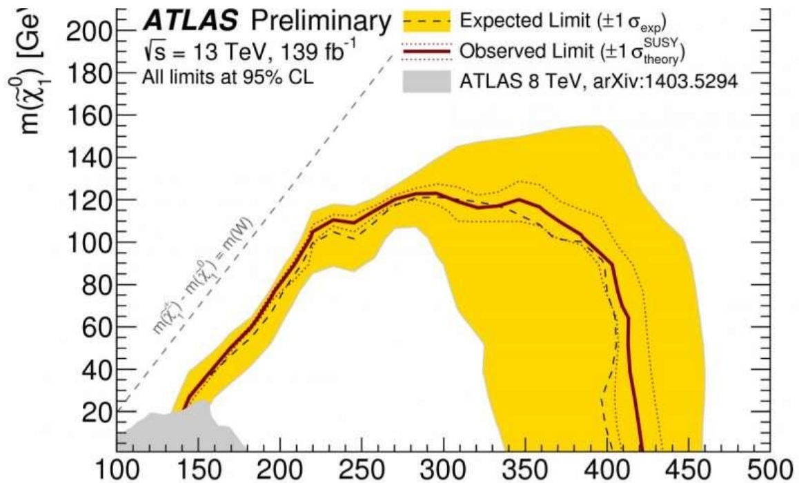
Figure 2: 95% exclusion limits on chargino pair production. The grey shaded region shows the results from Run 1 of the LHC. The new results substantially extend previous limits. Credit: ATLAS Collaboration/CERN
