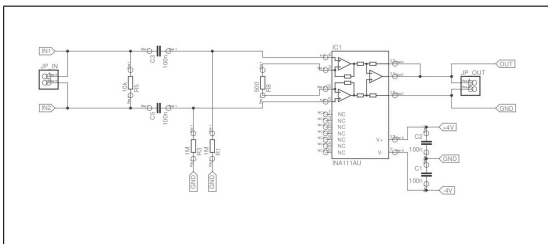
Figure 8: measuring amplifier
