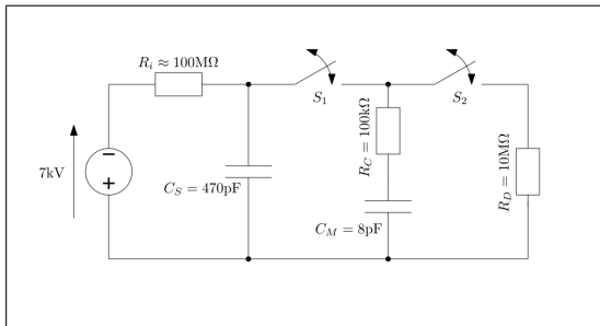
Figure 7: charging circuit
