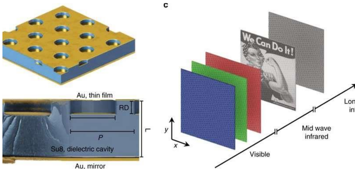
a) Schematic of the cavity-coupled plasmonic device consists of a backmirror, an imprinted array of holes in a polymer, and a second evaporation of gold to create disks and a perforated film. b) A false-colored scanning electron microscope ... more
