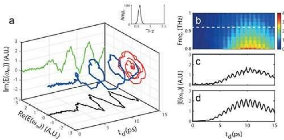
Figure 2. The complex amplitude of light at the converted frequency with the variation of a spatiotemporal boundary. Credit: The Korea Advanced Institute of Science and Technology (KAIST)
