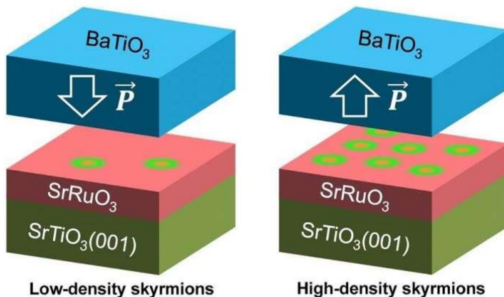
Figure 2: Controlling skyrmions' density with electric fields. This study measured skyrmions in an ultra-thin material made of a ferromagnetic layer of strontium ruthenate ( \text{SrRuO}_3 ), overlaid with a ferroelectric layer of barium titanate ... more
