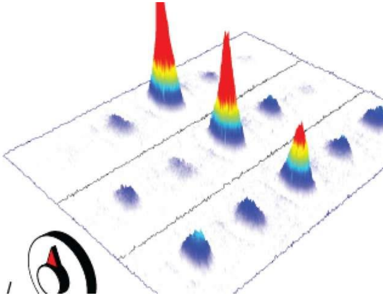
Images of the excited-state density distribution in the synthetic lattice for increasing magnetic flux values \Phi (increasing from left to right). Credit: F.A. An, University of Illinois at Urbana-Champaign
