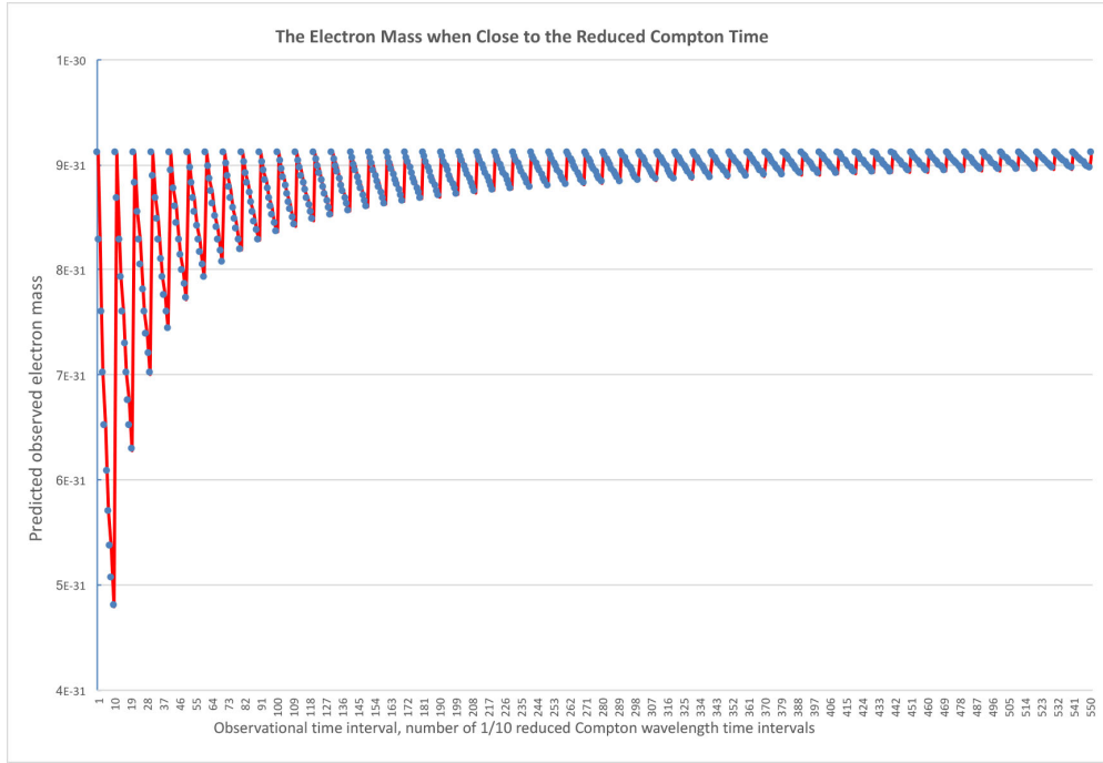
Figure 2: This figure illustrates the observation that the mass of an electron becomes time dependent at time intervals close to the reduced Compton time of the electron. The blue points are time points we have calculated for. The time intervals used are 0.1 reduced Compton time intervals.
