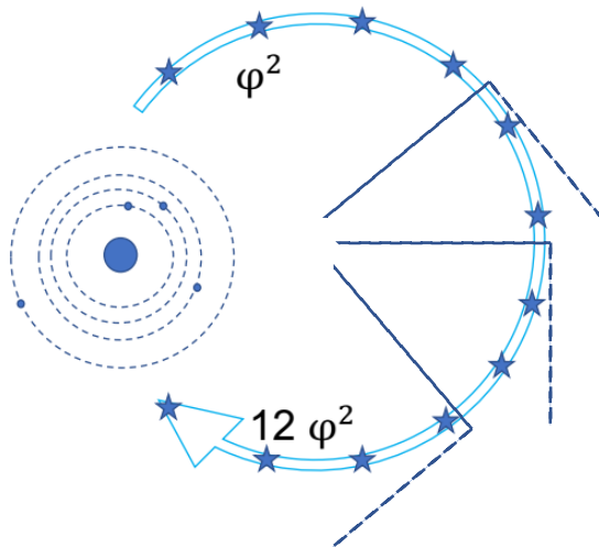
Figure 6: An atomic-styled solar-system platform with the CMBR from the entropic process of the sun reflected at right-angles in the stellar region, giving the effect of a “rotation” of light.
