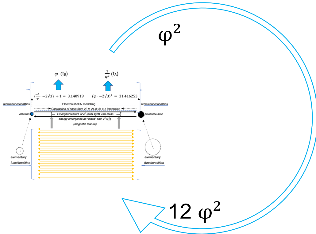
Figure 4: \varphi^2 \gg 12 \varphi^2 , (\varphi \cdot -2\sqrt{3})^2 , a process of the CMBR.
