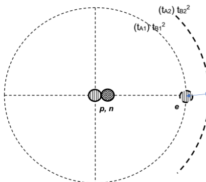
Figure 15.3.; both t_{A1} and t_{A2} represent a code relevant to the golden ratio that has already happened as a “past” event, thus we must create a new point source of light for t_{A1} and t_{A2} with this new t_{A2}-t_{A1} event.
