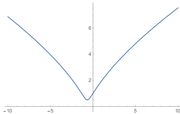
Figure 4. Plot of Ermakov-type solution for A=1, B=1
