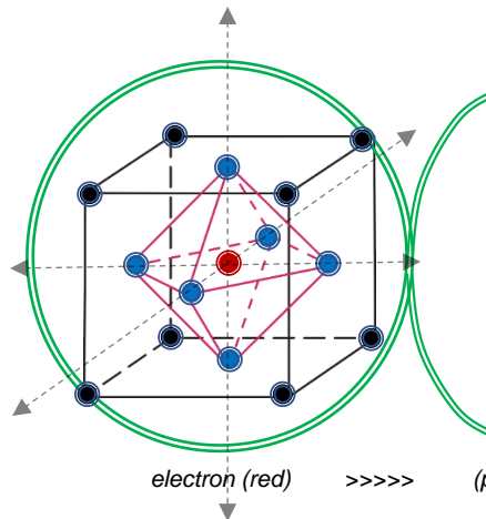
Figure 13: 15 particles/points, three zones: inner most 0-reference (red), middle octahedron (6-points, blue), outer cube (8-points, black). The proposal is the 0-reference is the electron, the middle-octahedron representative of either the generations (particle-spin) as “leptons” or the anti-quarks, and the outer-cube the 8 types of “anti-gluons” responsible for the “weak” nuclear force.
