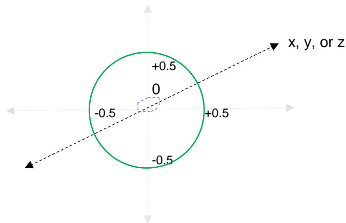
Figure 7; applying one time value to another, they are separated by a value of “1” circumscribing a circle around the x, y, or z axis.
