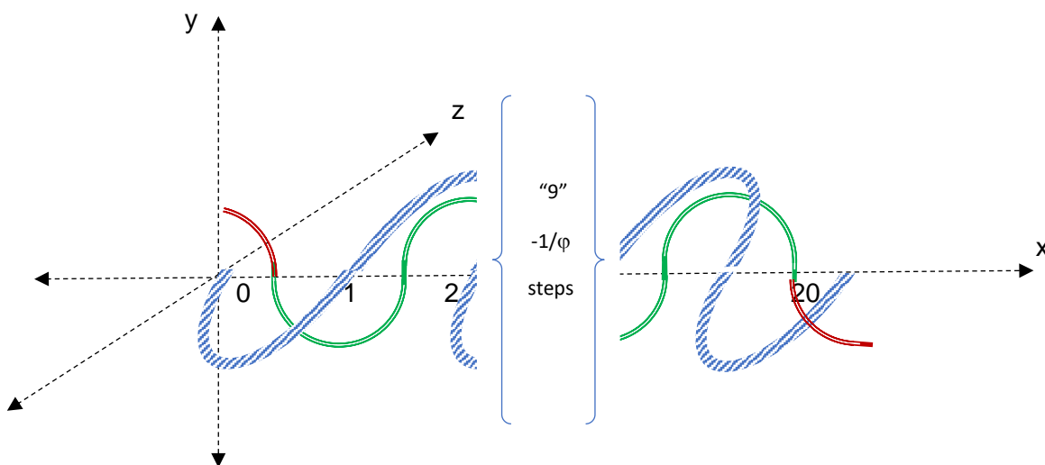
Figure 12; Green line electrical component (x,y), blue line magnetic component (x,z), both waves out of phase with each other and perpendicular to each other, magnetic wave used as the 0 start point extending 10 wavelengths ahead. Note the red line area though regarding the electrical component, and only 9 full electrical wavelengths have been completed, leaving another two partial wavelengths.
