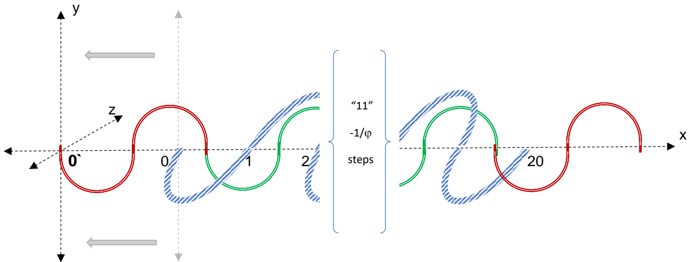
Figure 13; Note the addition of two extra wavelengths for the electrical component which by definition changes the 0-scalar spatial reference point of the wave by a measure of 3/2 .
