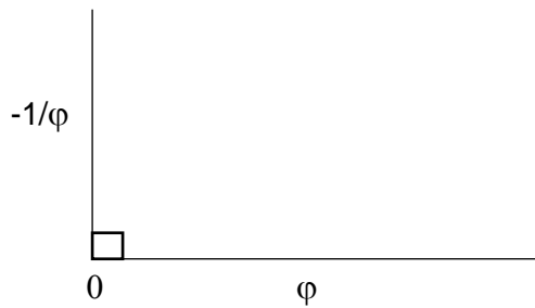
Figure 1; two axes of time, \frac{-1}{\varphi} and \varphi .
