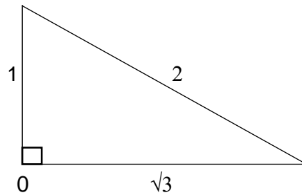
Figure 4; two axes of time, 1 and \sqrt{3} , which then result in the value of 2 in a squared relationship.
