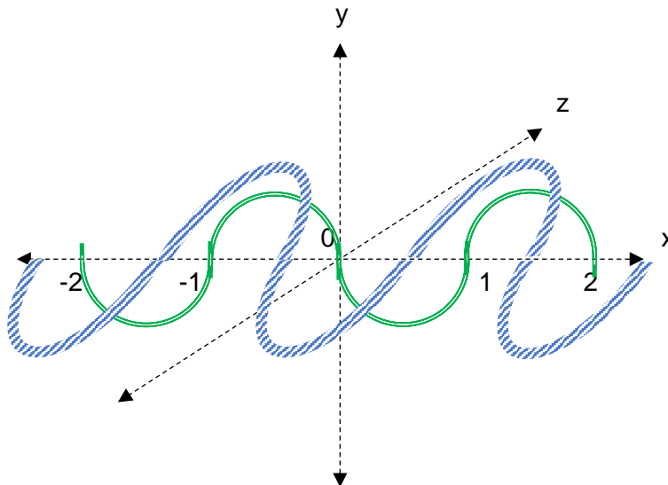
Figure 11.; Green line electrical component (x,y), blue line magnetic component (x,z), both waves out of phase with each other and perpendicular to each other.
