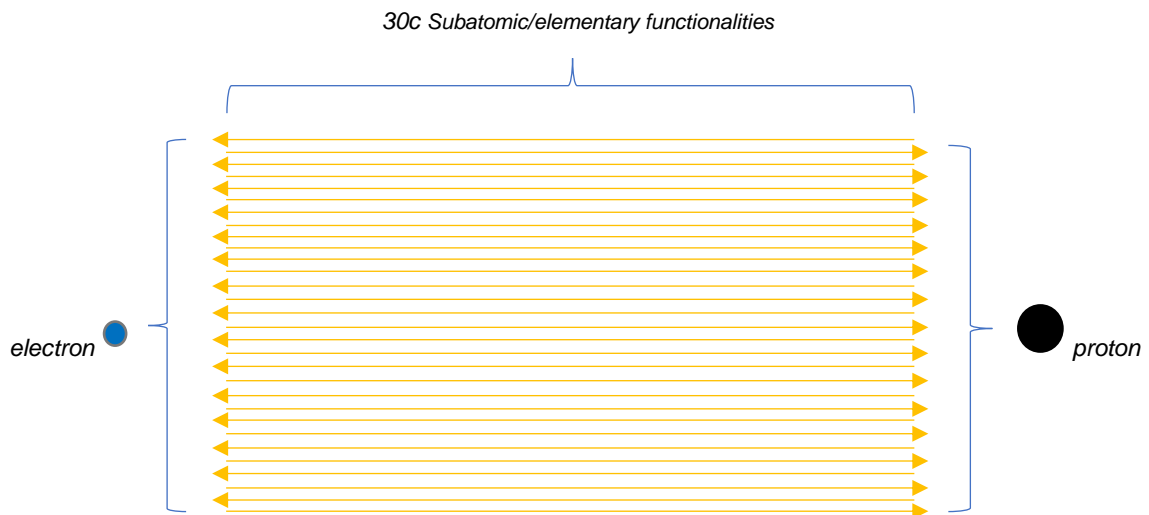
Figure 14; 15 “c” directions from the electron to the proton, and 15 “c” directions from the proton to the electron, each loop meriting a new unique status/orientation of the electron and proton.
