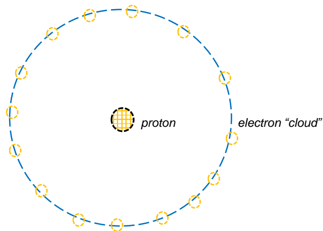
Figure 15; 15 “c” orientations for the electron to the proton, and 15 “c” internal sub-structure ingredients for the proton, once again each of the 30 “c” loops meriting a new unique status/orientation of the electron and proton.
