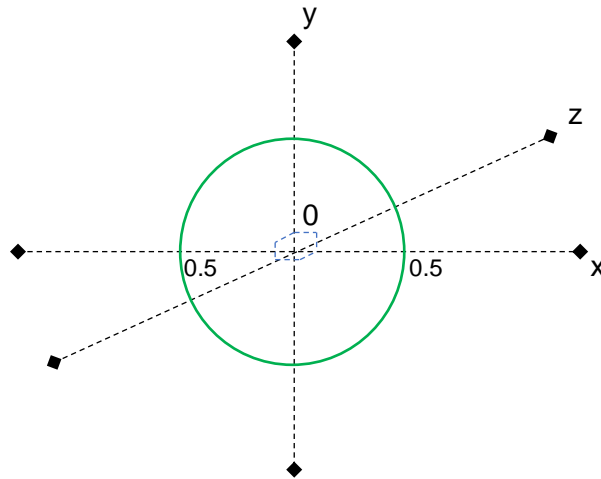
Figure 6; applying one time value to another, they are separated by a value of “1” circumscribing a circle around the z axis with a 0-scalar spatial central reference.
