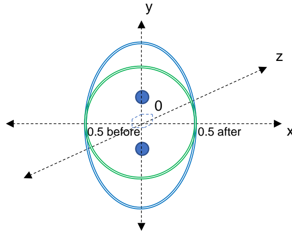
Figure 10; The circle ( \frac{1}{\phi} ) as the electrical component (green) is a circumferential value of \pi , the ellipse ( \phi ) as the magnetic component (blue) is a circumferential value of 4.6.
