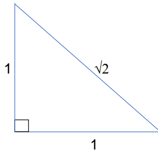
Figure 17; two axes of time t_N , 1 and 1, which then result in the value of \sqrt{2} in a squared relationship as a resultant value of t_N .
