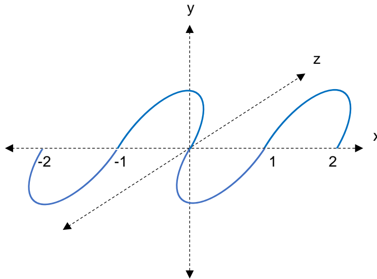
Figure 9; for the trace value of \varphi we would reach a value of 4.6 in each direction of the axis, the overall trace length for this sinusoidal wave would represent a value of 9.2 in factoring in the dual directions along the x-axis from the 0 reference.
