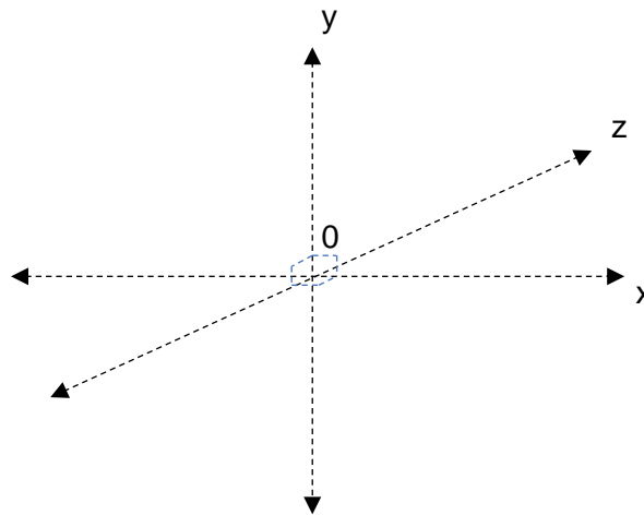
Figure 5; 3-dimensional ( 3 \cdot 1t_N space) dual directional space.
