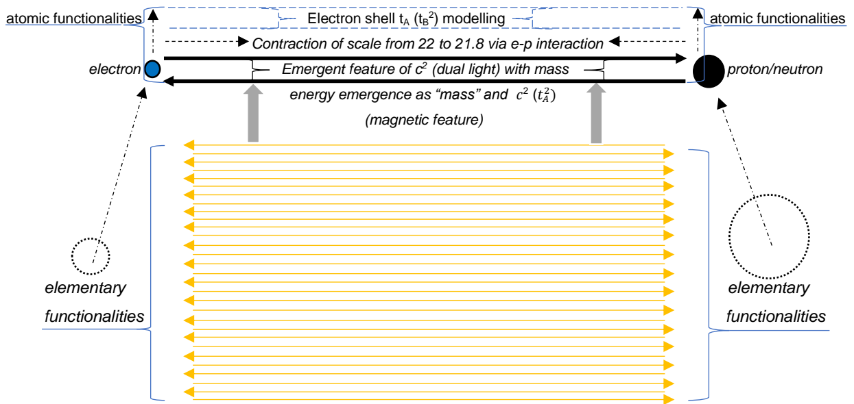
Figure 16; “beyond” the 30c manifold is a “c” factor that can only be “squared” as a “future” ( t_A^2 ) event beyond the primary 30c “now” event. Note also the contraction of the atomic scale from 22 to 21.8 owing to the emergent force between the electron and the proton, and subsequent electron shell modelling.
