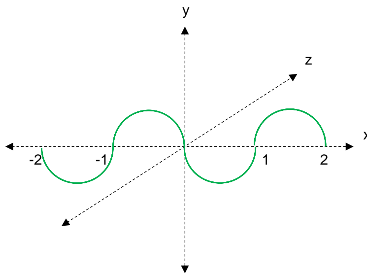
Figure 8; for the trace value of \frac{-1}{\varphi} we would reach a value of \pi in each direction of the x-axis, the overall trace length for this sinusoidal wave would represent a value of 2\pi in factoring in the dual directions along the x-axis from the 0 reference.
