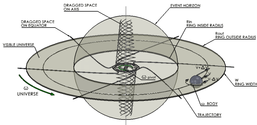
Fig. 4.2 - Structure and dimensions of the Pivot Universe
