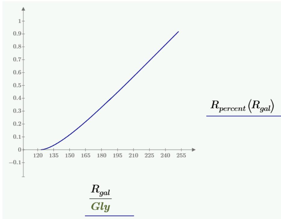
Fig. 8.2 - The ratio (%) of Doppler shift to the total z shift
