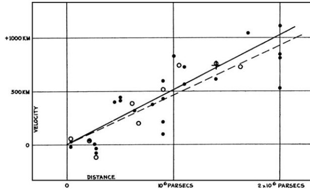
Fig. 8.1 – Hubble’s original graph (1929)
