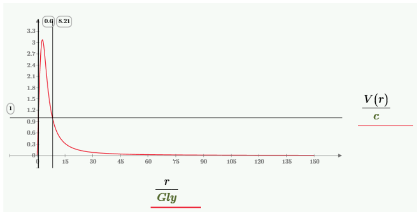
Fig. 4.1 – Velocity of dragged space around the Pivot
