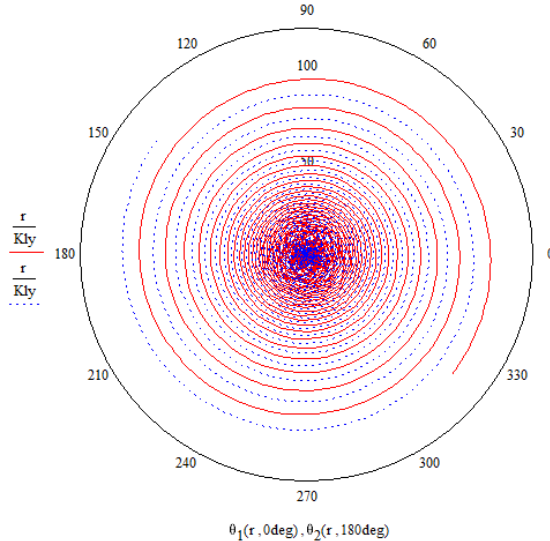
Fig. 9.3 – Shape of spiral Galaxy- 130 billion years after formation
