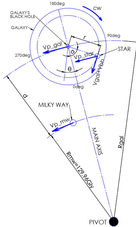
Fig. 8.1– Velocities of a star
