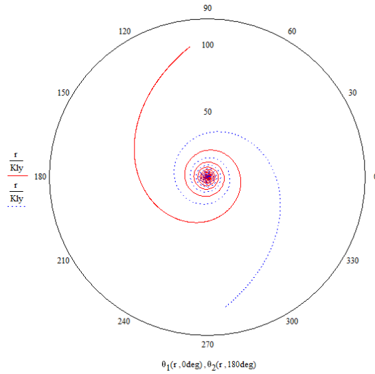
Fig. 9.1 – Shape of a current spiral Galaxy - 13 Billion years after its creation.
