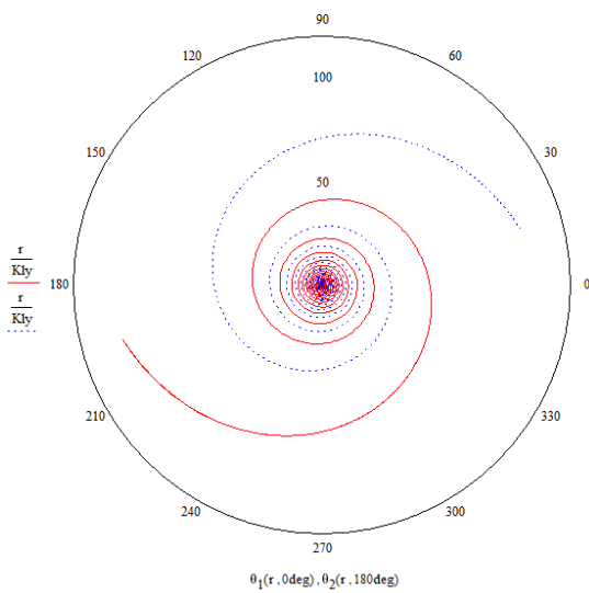
Fig. 9.2 – Shape of spiral Galaxy- 26 billion years after formation
