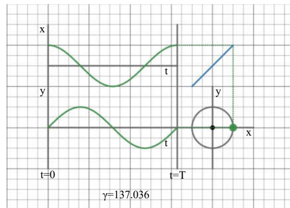
Figure 17 The Base Energy State
