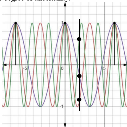
Figure 30 Uncertainty in the Third Energy State
