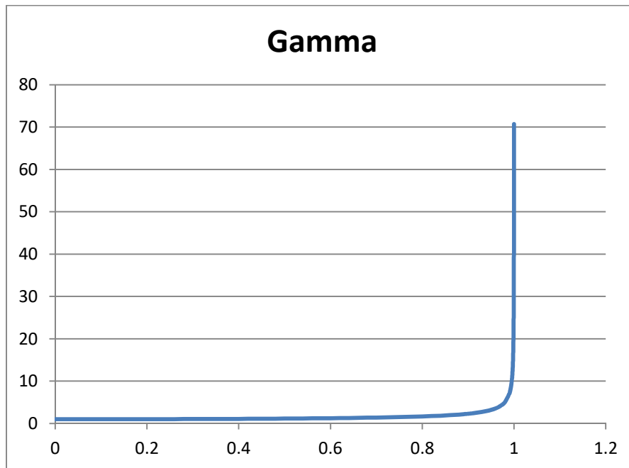
Figure 5 Graph of Gamma versus v/c
