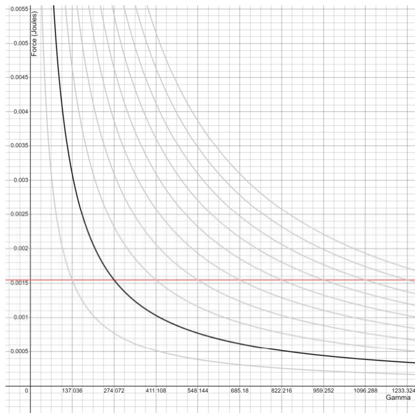
Figure 22 Family of Curves of Force vs Gamma
