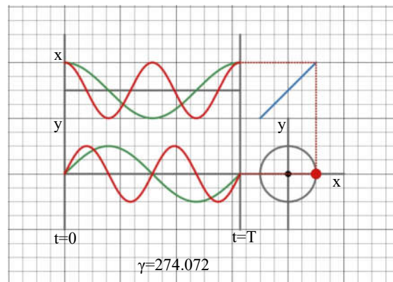
Figure 19 The Second Energy State
