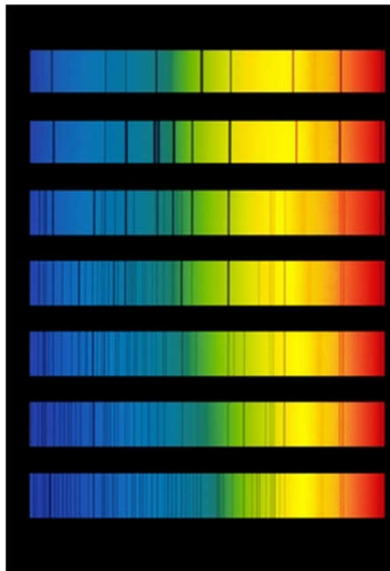
Figure 1 Absorption Spectra
