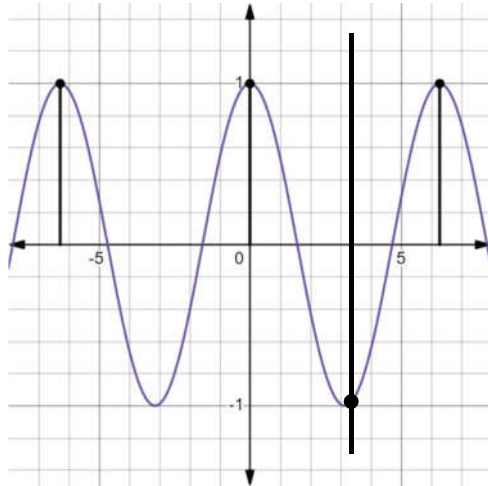
Figure 28 Uncertainty in the Base Energy State
