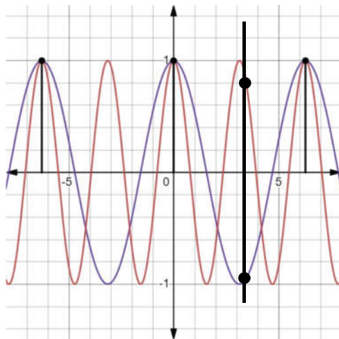
Figure 29 Uncertainty in the Second Energy State
