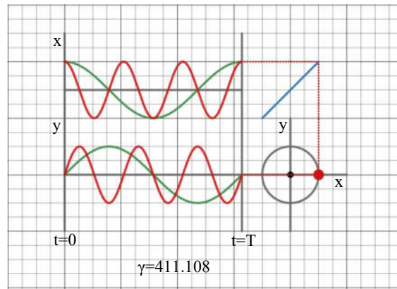
Figure 20 The Third Energy State
