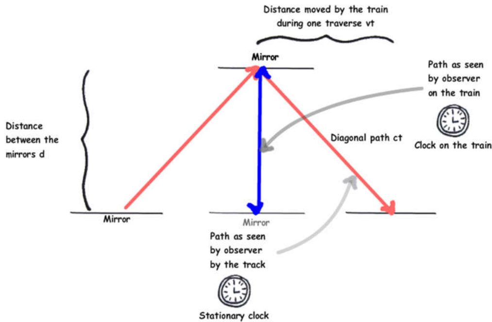
Figure 4 Special Relativity
