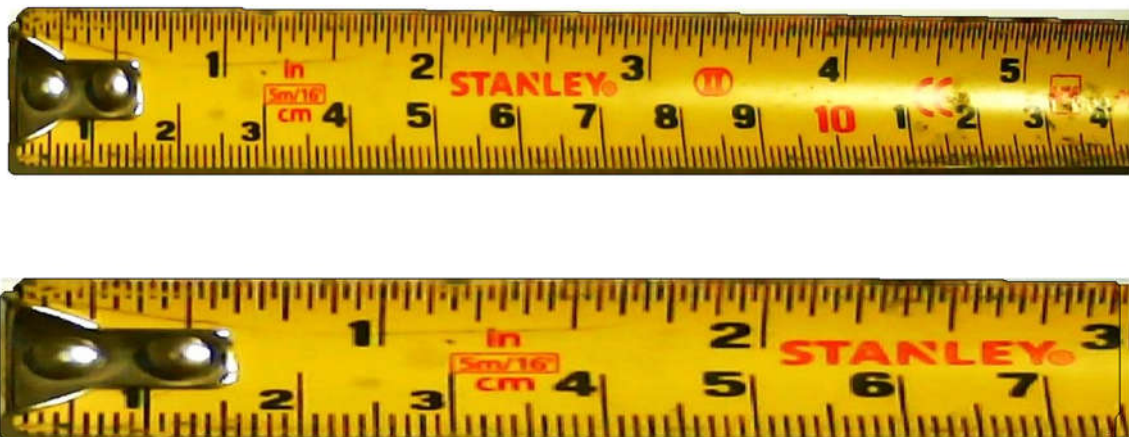
Figure 6 The Elastic Tape Measure
