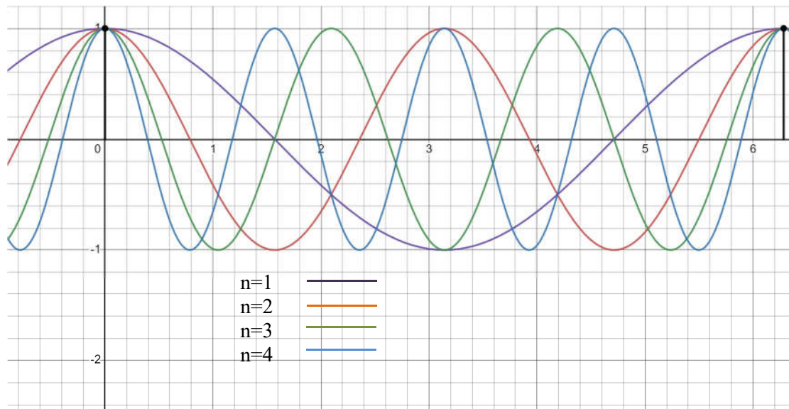
Figure 27 Electron Trajectories for n=1-4
