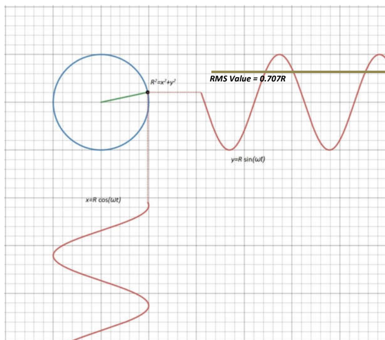
Figure 25 Parametric equations for the orbiting electron
