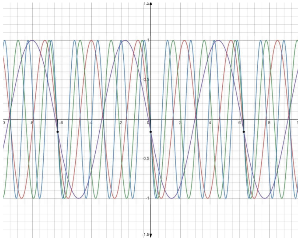
Figure 13 Sampling and Harmonics
