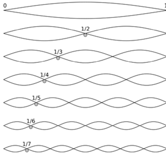
Figure 2 Standing Waves
