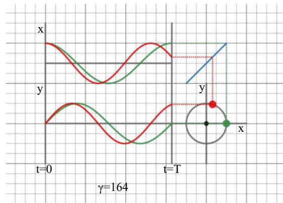
Figure 18 An Unstable State
