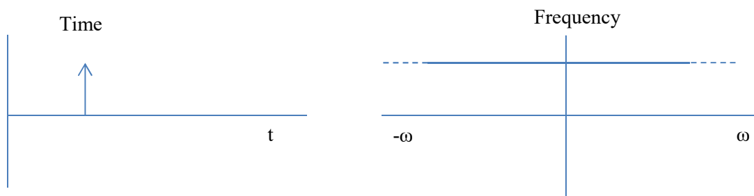
Figure 14 Fourier transform of a single Dirac function
