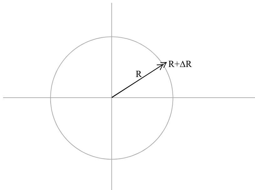
Figure 23 A small change in orbital radius
