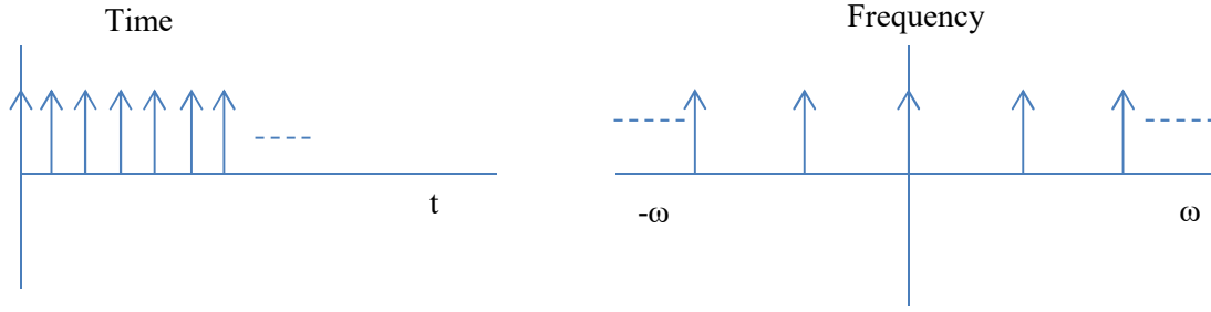
Figure 16 Fourier transform of a higher frequency Dirac comb
