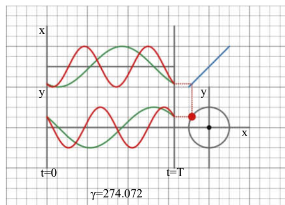
Figure 21 The Effect of a Phase Shift
