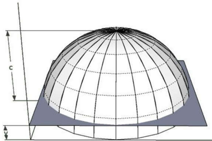
Figure 8 Spherical representation of a circular orbital path under relativity
