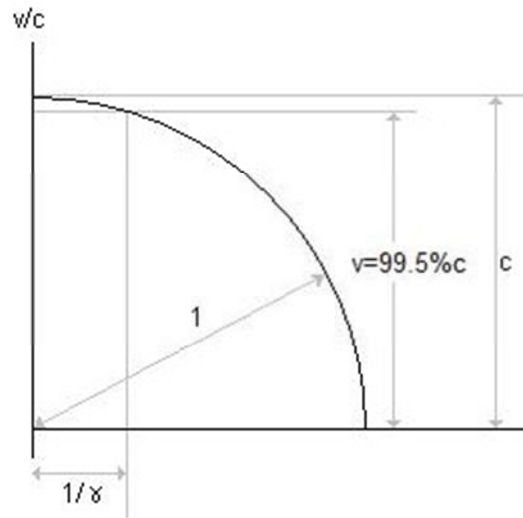
Figure 7 Reciprocal of Gamma
