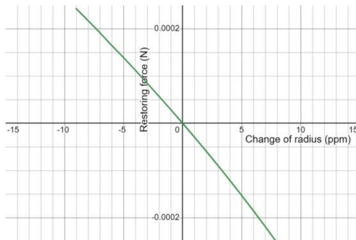
Figure 24 Restoring force vs Change of Radius
