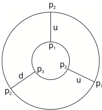
Fig. 2. Pictorial representation of the arrangement of primons in the proton. In the neutron the inner layer is the same, and in the outer layer the p_1 below is replaced by p_3 and this makes the neutron to be udd in terms of quarks.
