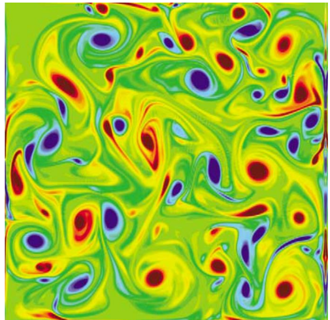
Fig. 3. How the vorteons and the fluid of nucleons and electrons inside each cluster of galaxies will look like after galaxies lose their outskirts due to the shrinking of the cluster by its gravity. Galaxies will be reduced to rotating spheroids of nucleons, which we may call vorteons. In this figure the vorteons are the roundish blue and red bodies. The figure is from an article by Clercx et al. [87] on turbulence in two dimensions in square and circular domains (figure used by permission).
