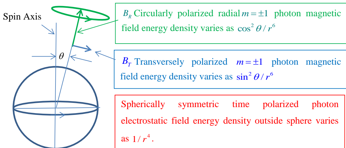
Figure 2.3. 1 Spinning electrically charged sphere. At the same radius B_R (@ \theta = 0) = 2B_T (@ \theta = \pi / 2)
