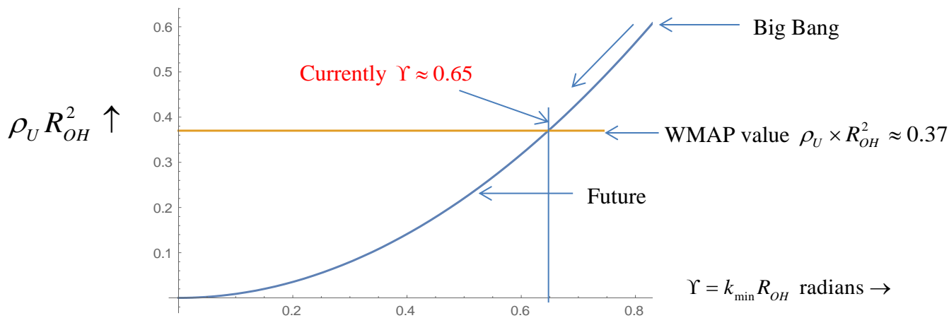
Figure 2.4. 2 plots \rho_U \times R_{OH}^2 \approx 0.8823\Upsilon^2
