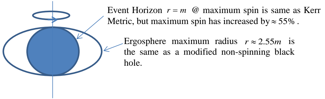
Figure 2.6.1 Modified Kerr Metric with the dimensionless parameter A changed from A = \frac{2m}{r} \rightarrow A = \frac{2m}{r} + 1.39 \frac{m^2}{r^2} . This conflicts with General Relativity near the horizon.
