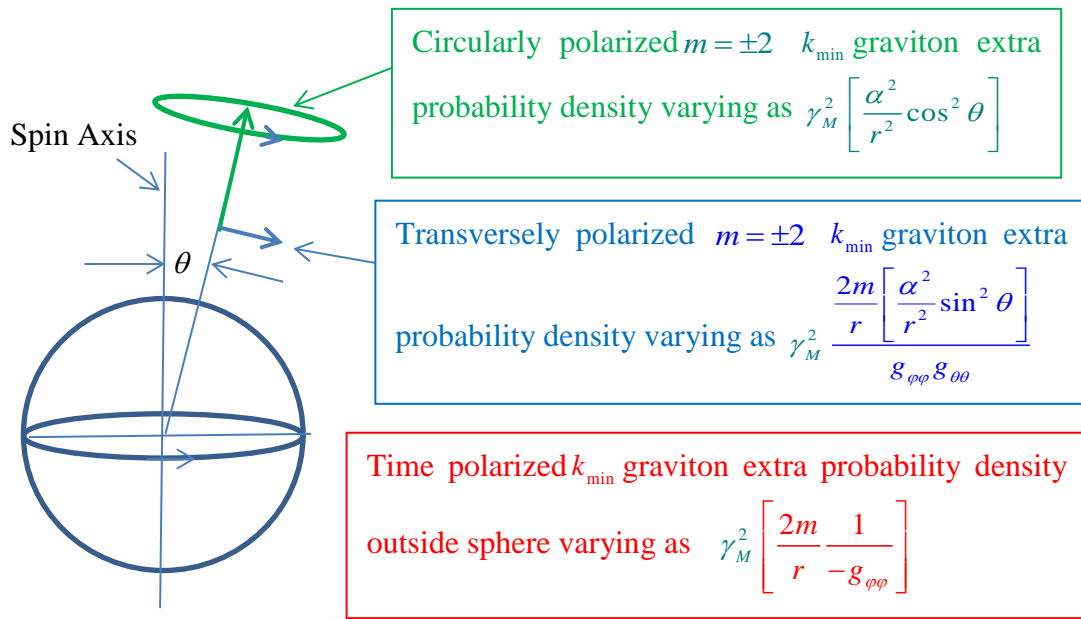
Figure 2.3. 2 Spinning mass m with angular momentum length parameter \alpha . The time polarized k_{\min} gravitons are distorted from spherical symmetry as -1/g_{\varphi\varphi} . For r \gg r_{Sw} we can ignore the effects of g_{\theta\theta}, g_{\varphi\varphi} & \gamma_M^2 , as all three rapidly tend to \pm 1 when written in dimensionless form as in Equ's.(2.3. 2). These values are the extra probability densities before the density dilution due to the expansion of space around the rotating mass.
