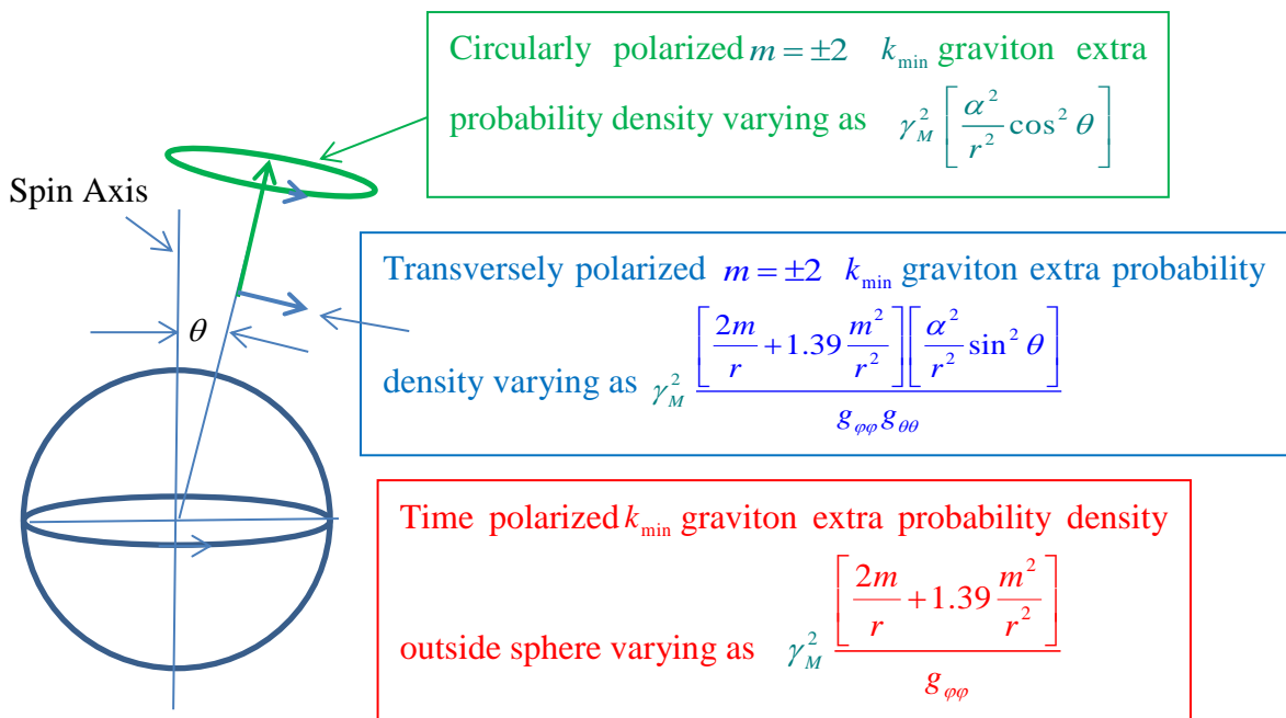
Figure 2.6.1 Modified Kerr Metric with the dimensionless parameter A changed from A = \frac{2m}{r} \rightarrow A = \frac{2m}{r} + 1.39 \frac{m^2}{r^2} . This conflicts with General Relativity near the horizon.
