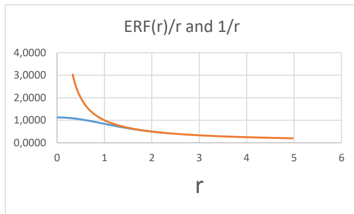
Figure 1. Close to the geometric center, the singularities convert into a smooth function. Farther from the center, the function retains the form of the Green's function (1/r).
