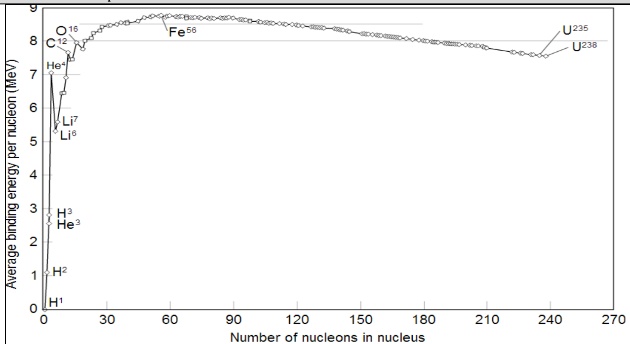
Figure F5-1. E_{BN} ([average] nuclear binding energy [per each nucleon]) variation with the nof. nucleons ( N_{anc}=N_{ap}+N_{an} ) [30]
