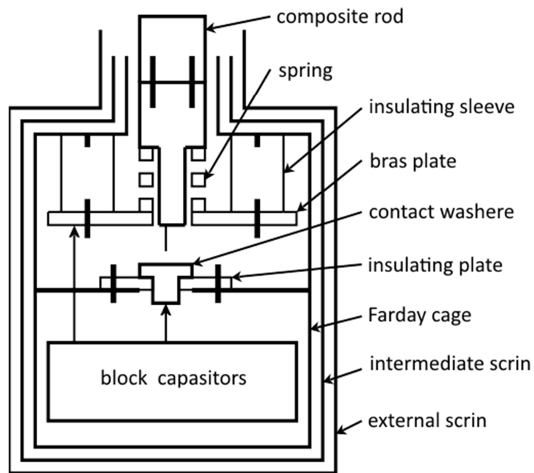
Fig. 20. The schematic of experimental installation.
