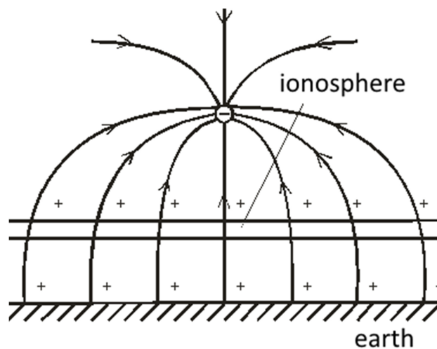
Fig. 33. Negative charge above the earth's surface with the presence of the ionosphere.
