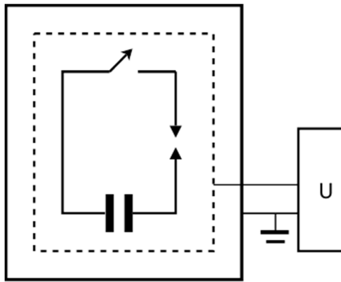
Fig. 18. Diagram of experiment with one external screen.
