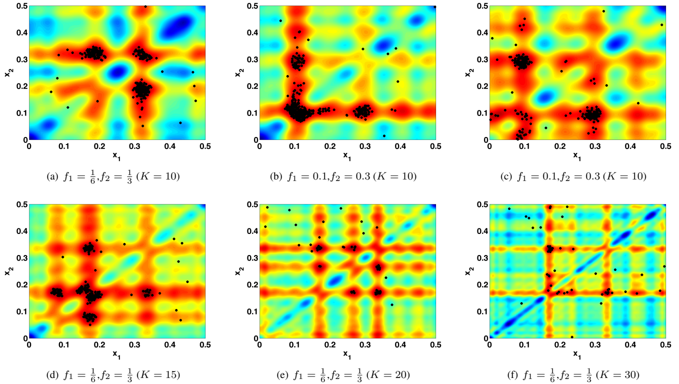
Fig. 5. Several examples of function V(\mathbf{x}) = \log \pi(\mathbf{x}) with S = 2 , given different realizations of the measurements y[1], \dots, y[K] . In Figures (a)-(d)-(e)-(f), we set \mathbf{f} = [\frac{1}{6}, \frac{1}{3}]^\top and consider K = 10, 15, 20, 30 , respectively. In Figures (b)-(c), we set \mathbf{f} = [0.1, 0.3]^\top and K = 10 . Black dotted points shows all the states generated throughout an O-MCMC-PMTM run with N = 10, L = 10 and T = 500 . The initial states are chosen uniformly within \mathcal{D} = [0, \frac{1}{2}]^\top .
