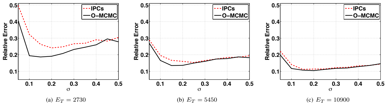
Fig. 6. Relative Error (averaged over 500 runs) in the first experiment for O-MCMC-SMH (solid line) and IPCs (dashed line) with different computational effort E_T . Note that O-MCMC always outperforms IPCs. Note also that their performance becomes similar as the overall computational cost E_T grows (due to the small size of the state space, \mathcal{D} = [0, \frac{1}{2}]^2 ).
