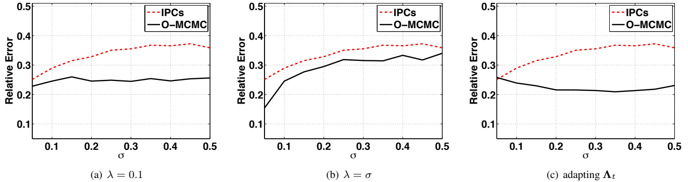
Fig. 7. Relative Error (averaged over 500 runs) in the second experiment (dimension S = 4 ) searching the global maximum with O-MCMC (solid line) and IPCs (dashed line). In the O-MCMC-PMTM scheme, we use different \lambda = 0.1 and \lambda = \sigma , for the covariance matrices \Lambda_n = \lambda^2 \mathbf{I}_4 of the horizontal proposal pdfs in the mixture \psi . Moreover, we test an adapted covariance matrices for the horizontal proposal pdfs (see Figure (c)).
