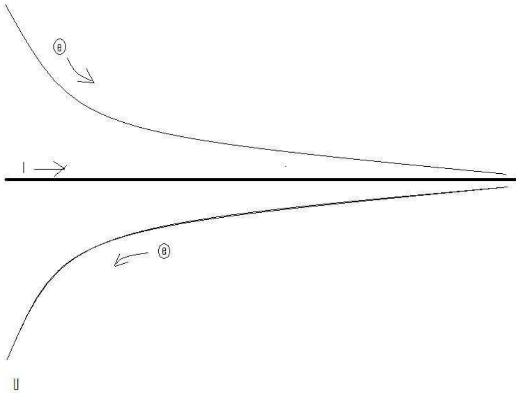
Figure 3.) Concentric 1/x equipotential surfaces around the electric wire causes the magnetic effect on the external moving charges
