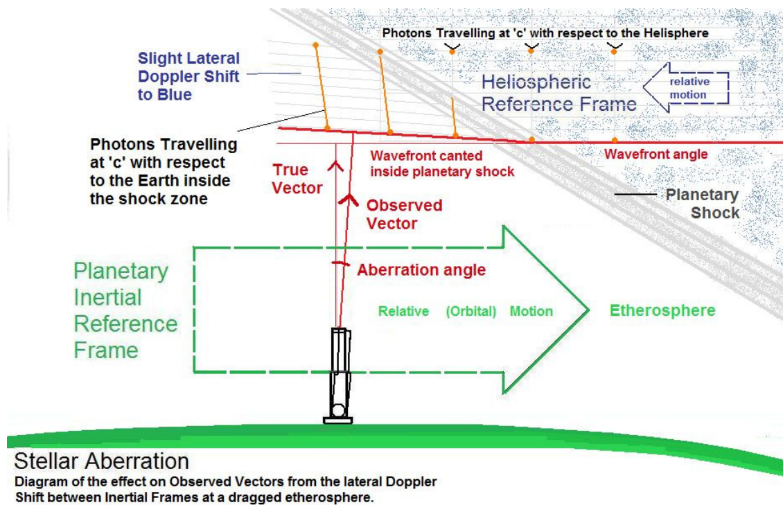
Fig 4. Stellar Aberration; Canting of the wave front. (due to relative motion of the media).
