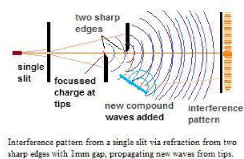
Figure 10c. Fine interference from tip wave propagation. The lack of back waves in HFP is suggested as due to conserved 'spin' signal.
