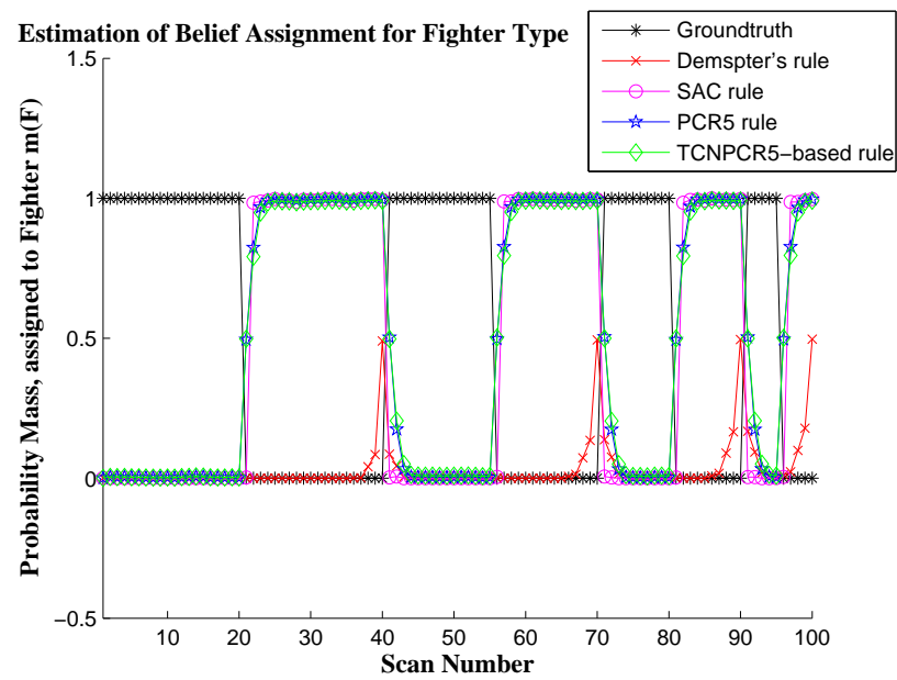
Figure 13.9: Belief mass for Fighter Type, T -variable step, case 1
