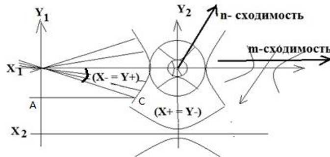
Fig. 3a. dynamic space-matter
