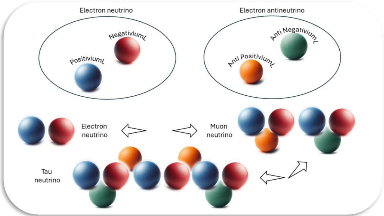
Figure 1 Neutrinos oscilations
