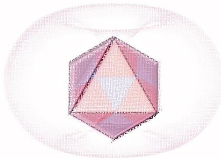
Figure 3.2 - The neutron (0)
