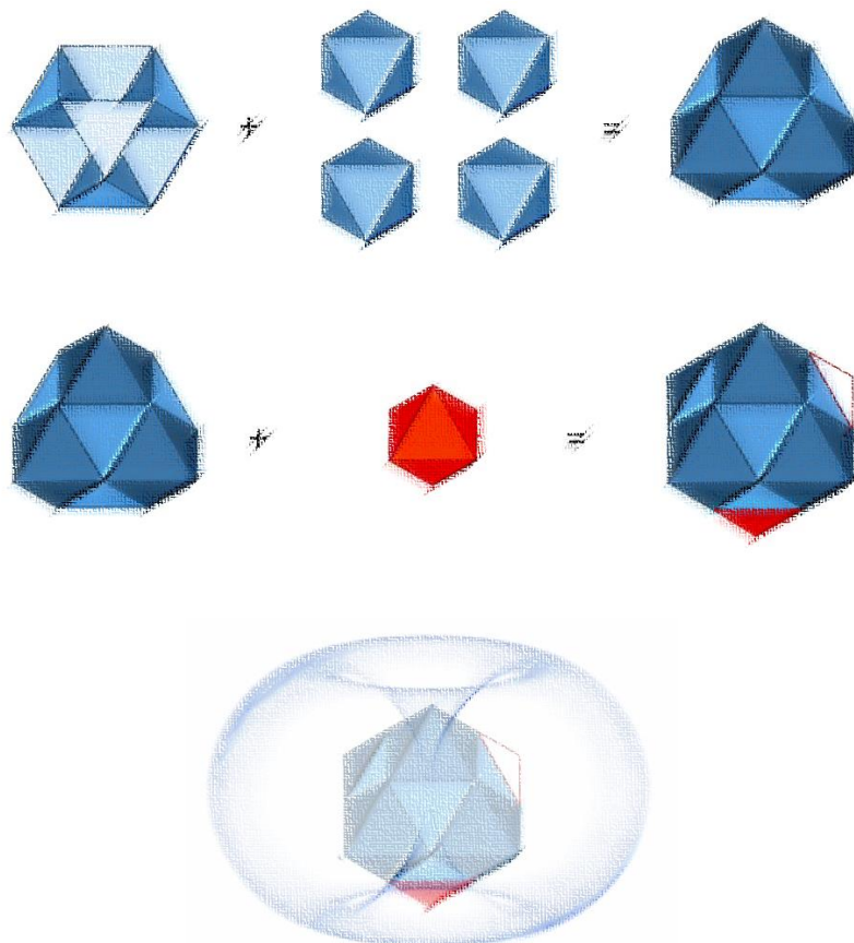
Figure 3.3 - The Proton (+1)
