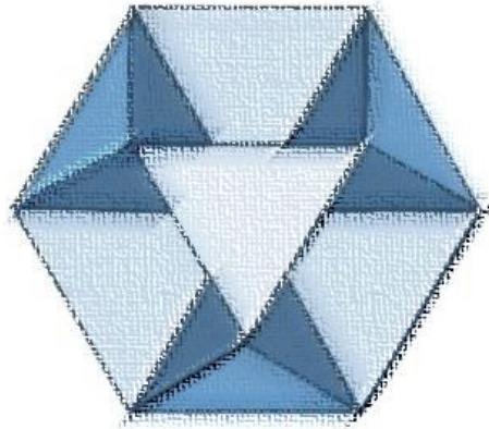
Figure 2.8 - Octahemioctahedron
