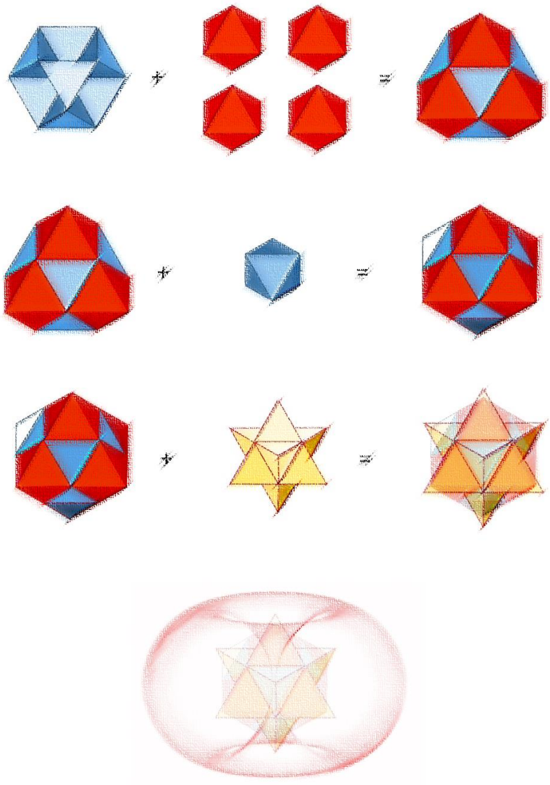
Figure 3.4 - The Electron (-1)
