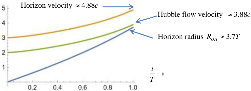
Figure 8.2. 2 A plot of the k = 0.009 solution with H_0 = 73 \text{ km/sec/Mps} .
