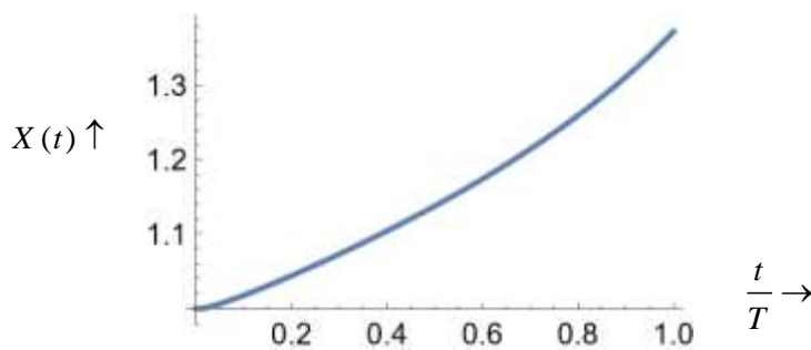
Figure 8.2.6 A plot of X(t) as in Equ's.(8.2.3) & (8.2.13). The massive graviton coupling parameter \alpha_{MG} , that increases as the square of the mass ratio of massive gravitons plus baryons, is the above curve squared i.e. X(t)^2 , with X(t = 1)^2 \approx 2 currently.
