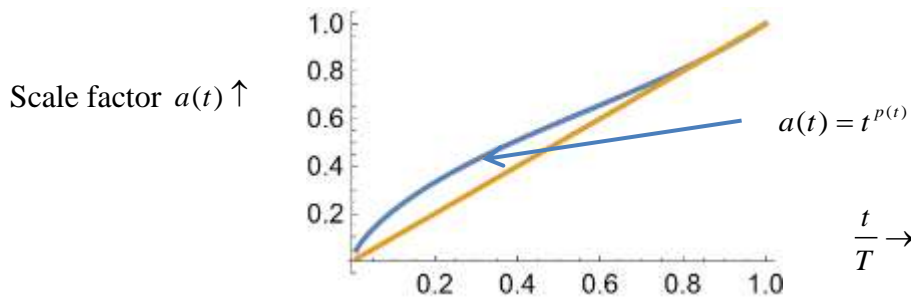
Figure 8.2.4 A plot of the k = 0.009 scale factor showing similar behaviour to the Lambda-CDM.
