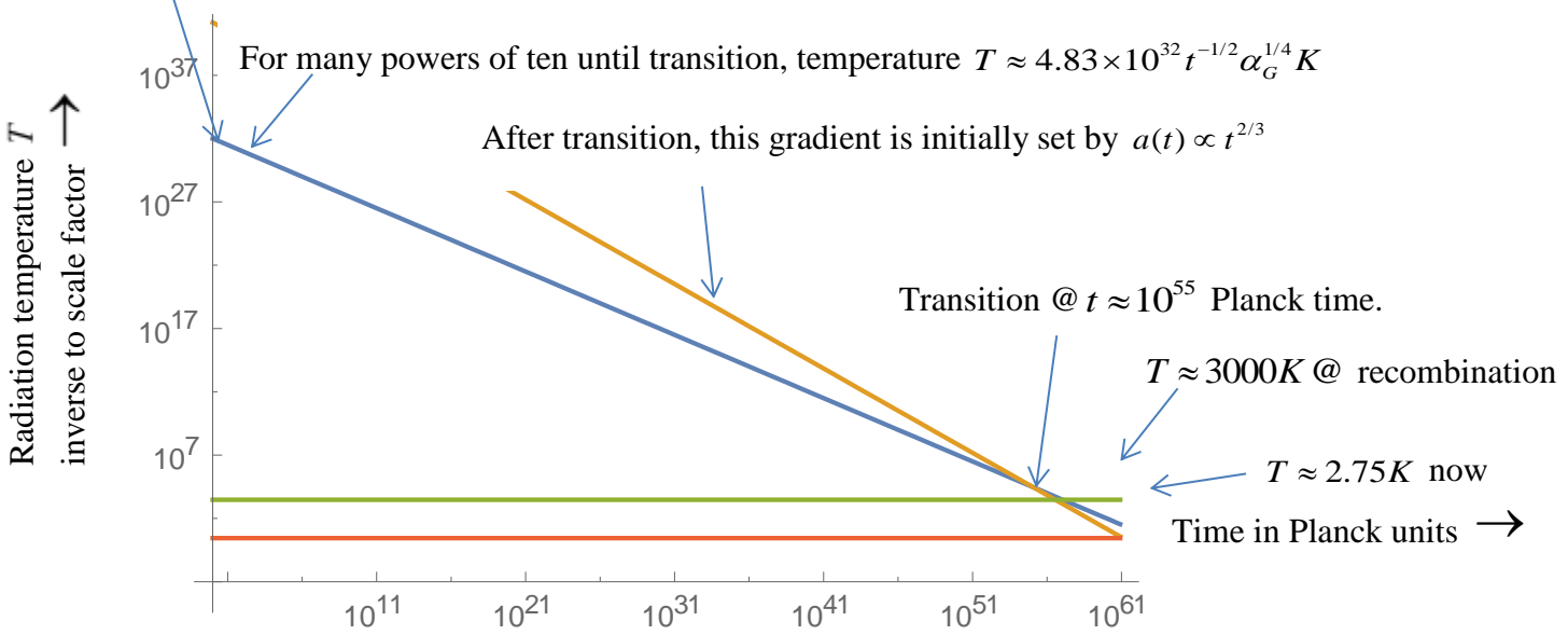
Figure 5.3.2 A logarithmic temperature plot with \alpha_G = 0.018 from t \approx 2 Planck units until now.
