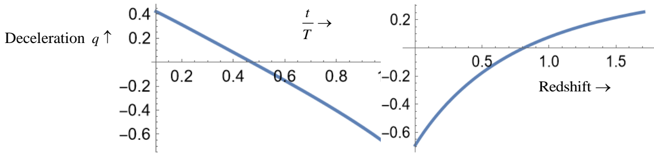
Figure 8.2.3 A plot of deceleration parameter q versus time on the left, and versus redshift z on the right, for the k = 0.009 solution.
