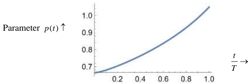
Figure 8.2.5 The behaviour of the parameter p(t) for the k = 0.009 solution.
