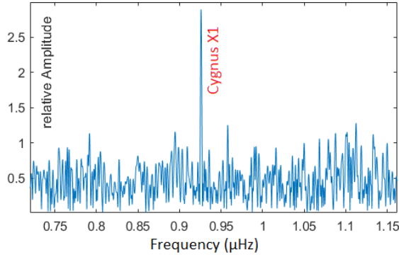
Figure 1): Spectrum of the GW of Cygnus X1 after changing the frequency to f_{ZF} = 1/(300 \text{ hours}) and compensating the phase modulations. This increases the amplitude of the carrier frequency of the GW significantly. The vicinity of f_{ZF} is filled with the distorted spread spectra of previously undiscovered GWs of similar frequency.
