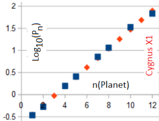
Figure 2): The logarithm of the orbital period of the planets (in years) of Cygnus X1 as a function of their order. The actual values (blue) hardly differ from Dermott's law (red). Despite an intensive search, the PM of the "missing" planets could not be detected.
